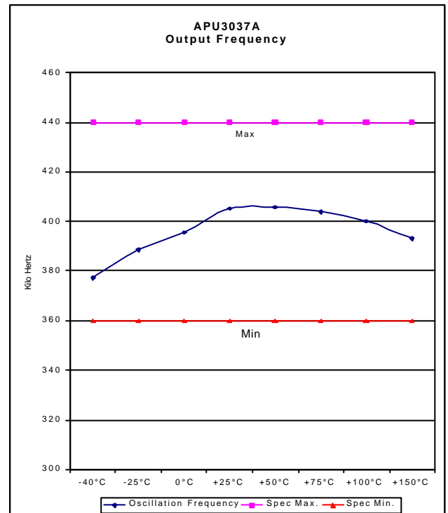
Figure 15 - Output Frequency
