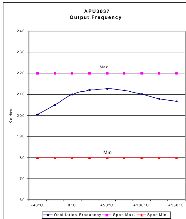
Figure 12 - Output Frequency
