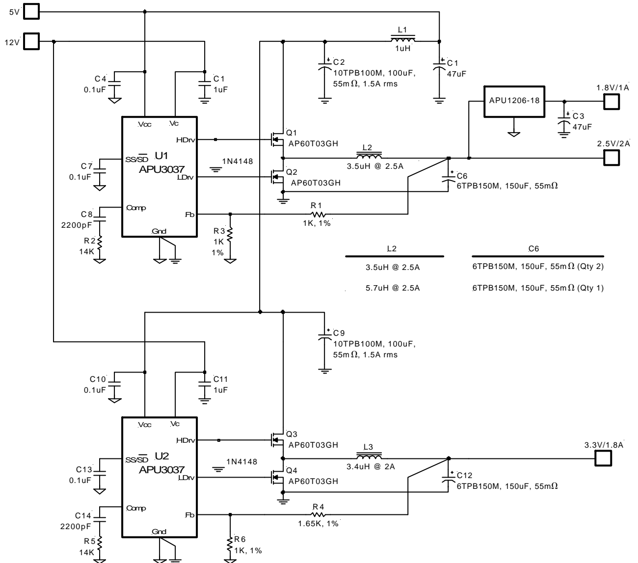
Figure 19 - Typical application of APU3037 or APU3037A in an on-board DC-DC converter providing the Core, GTL+, and Clock supplies for the Pentium II microprocessor.
