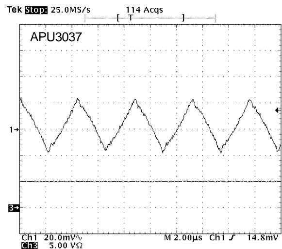
Figure 25 - 3.3V output voltage ripple @ I_{OUT}=5A .
