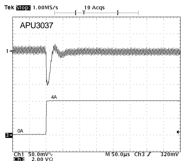
Figure 27 - Transient response @ I_{OUT} = 0 to 4A.
