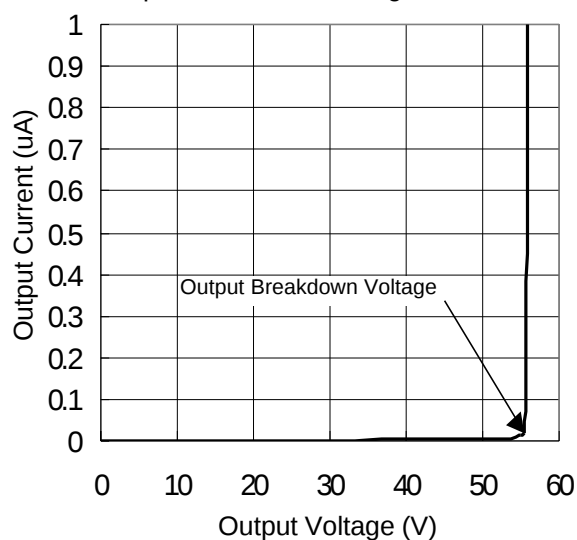
Output Breakdown Voltage vs. Current
