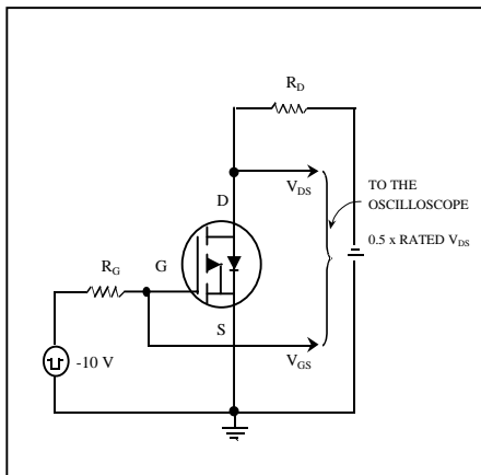
Fig11. Switching Time Circuit
