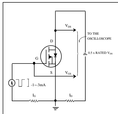
Fig 12. Gate Charge Circuit
