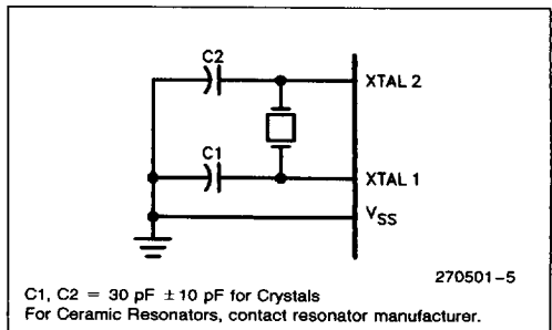
Figure 4. Oscillator Connections
