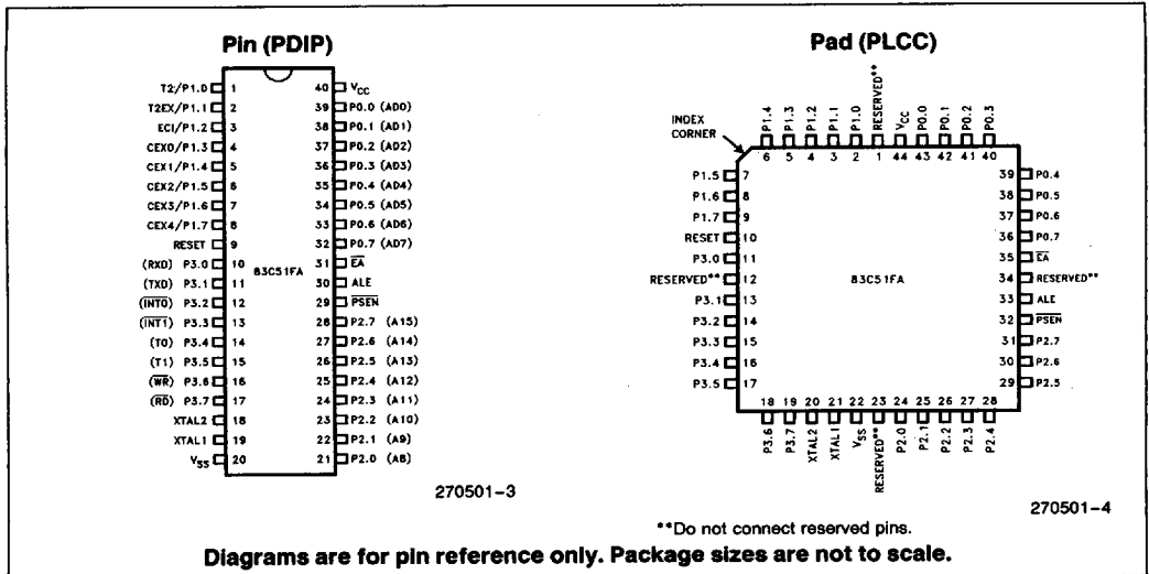
Figure 3. Pin Connections
