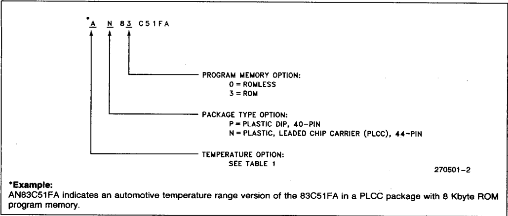
Figure 2. MCS® 51 Microcontroller Product Family Nomenclature
