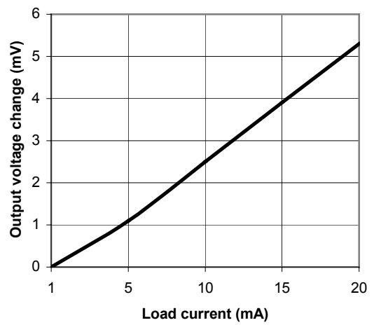
Load regulation
