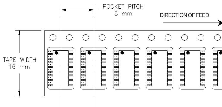
Figure 22: Tape Dimensions
