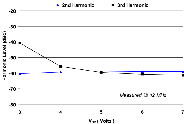
Figure 10: Harmonic Distortion vs V_{DD} P_{OUT} = 58\text{dBmV}
