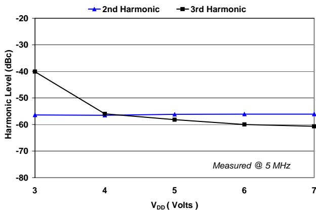
Figure 10: Harmonic Distortion vs V_{DD} P_{OUT} = 58\text{dBmV}
