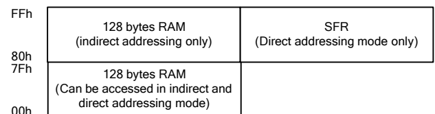
FIGURE 4: VRS51x540 DATA MEMORY
