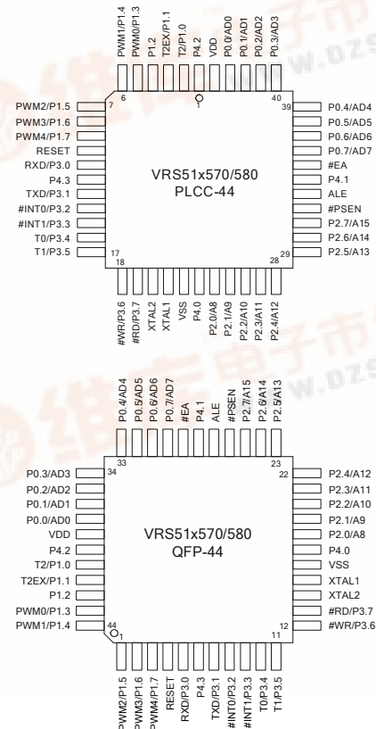
FIGURE 2: VRS51x570 / VRS51x580 PLCC AND QFP PINOUT DIAGRAMS
