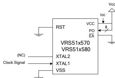
FIGURE 23: ICC IDLE MODE TEST CIRCUIT
