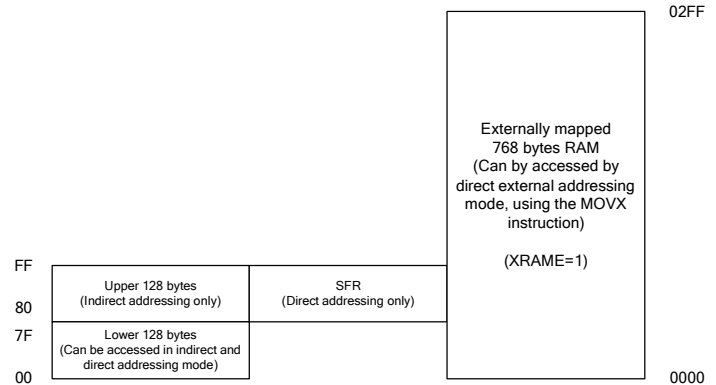
FIGURE 4: VRS51x570 /VRS51x580 RAM MEMORY
