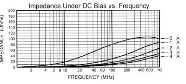
MLB-321611-0090PQ
