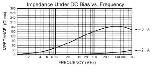
MLB-321611-0500PP
