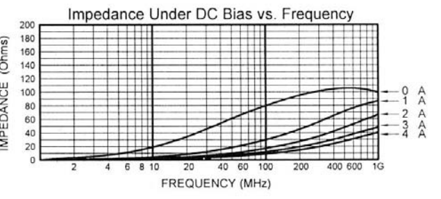
MLB-321611-0080PR
