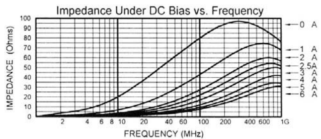
MLB-451616-0080PW
