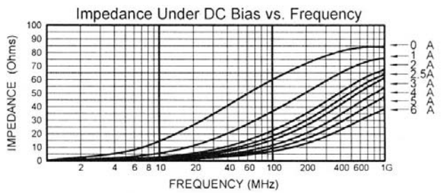
MLB-451616-0060PW
