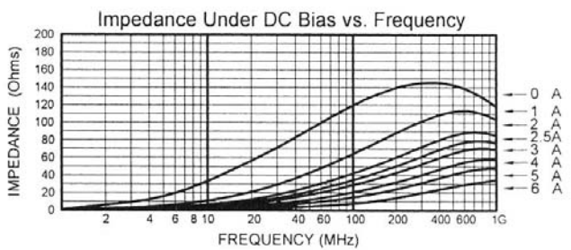
MLB-453215-0120PW
