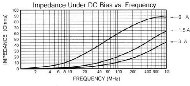
MLB-321611-0060PQ
