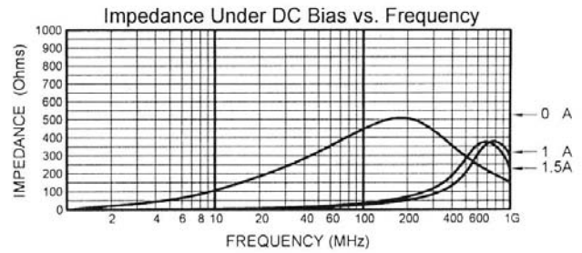
MLB-160808-0450PM
