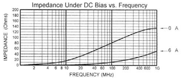
MLB-453215-0080PW
