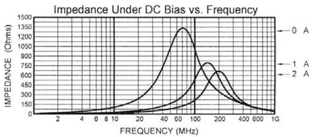
MLB-322513-1000PN
