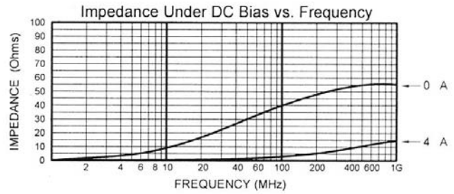
MLB-201209-0040PR
