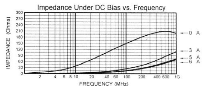
MLB-453215-0150PW
