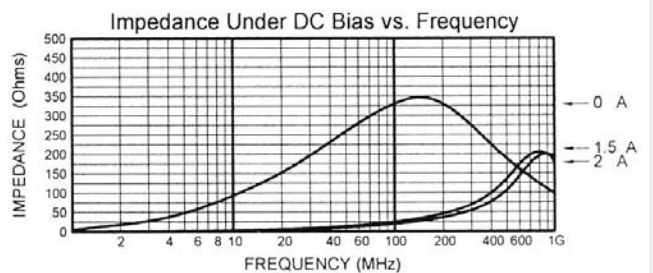
MLB-201209-0600PN
