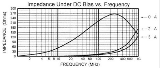
MLB-201209-0220PQ
