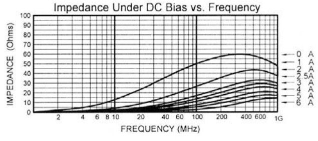
MLB-321611-0050PW
