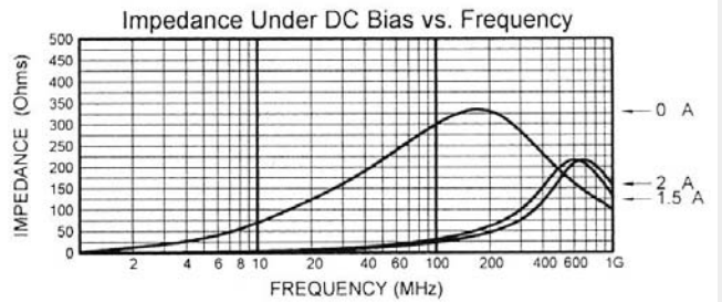
MLB-201209-0300PN
