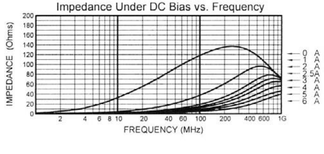
MLB-321611-0150PN
