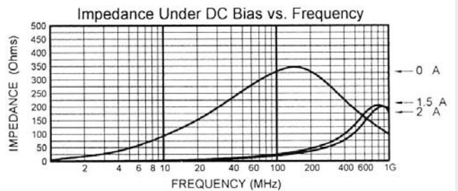
MLB-201209-0330PN
