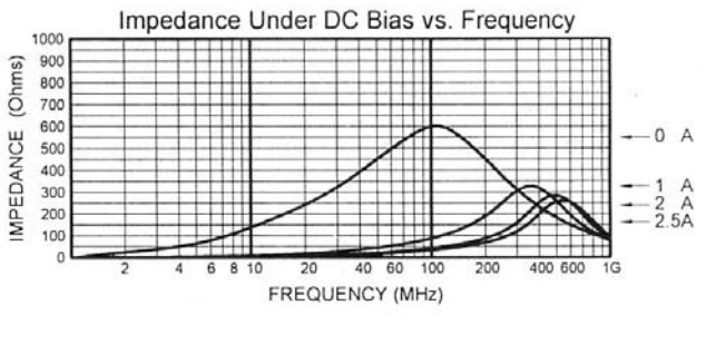
MLB-321611-0600PP
