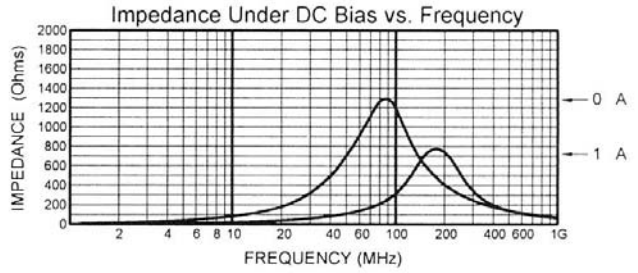
MLB-321611-1200PL
