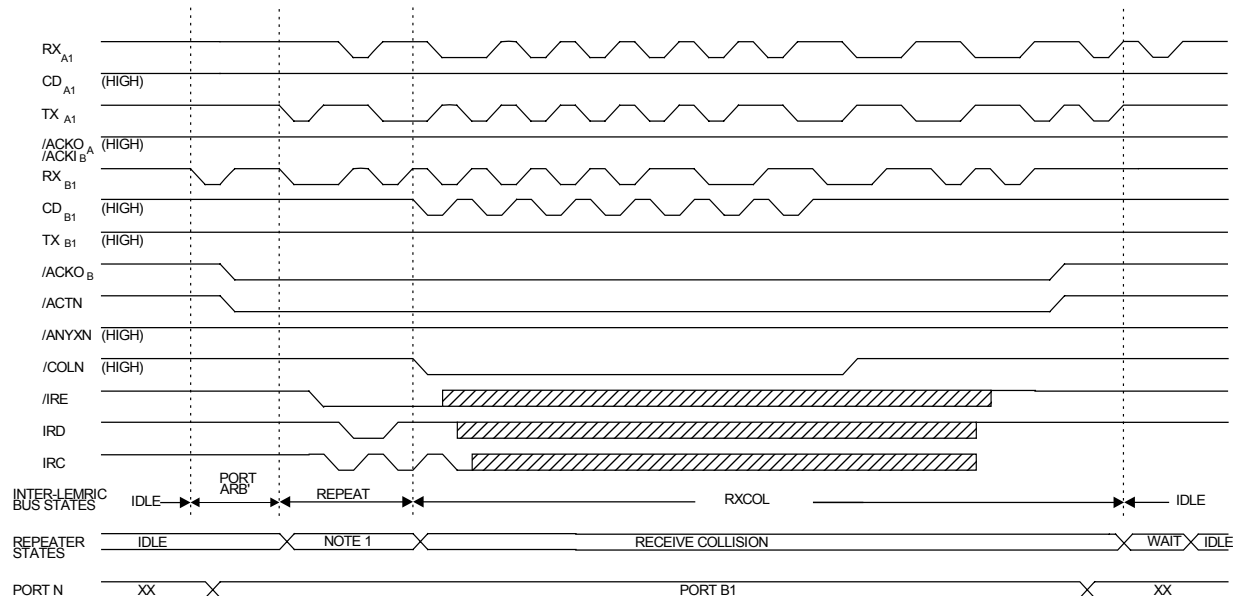
FIGURE 11. Receive Collision
