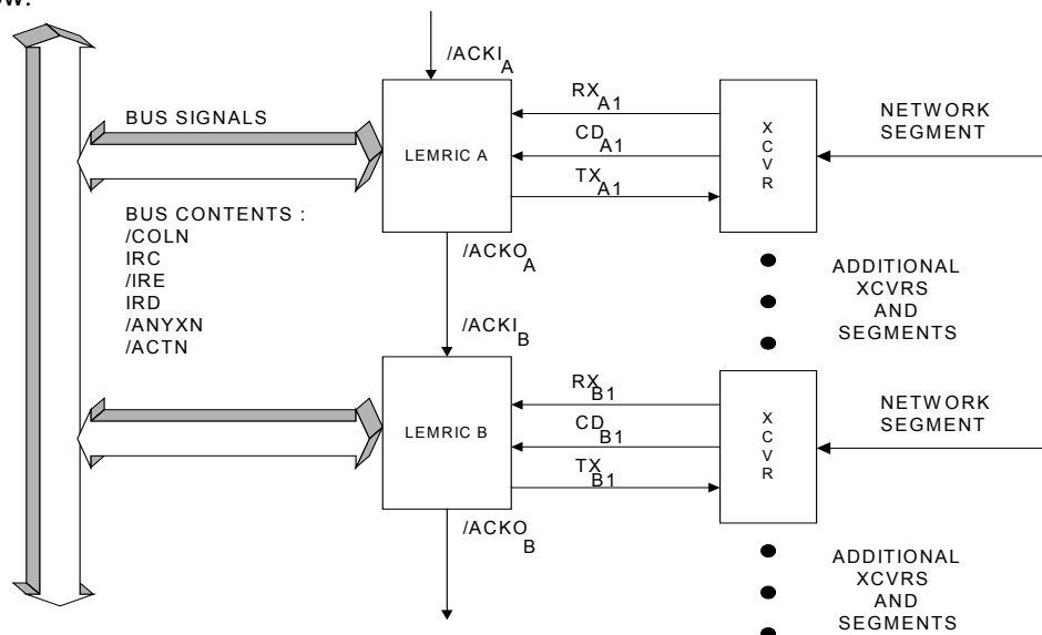
Figure 9. MULTI-LEMRICs System Topology
