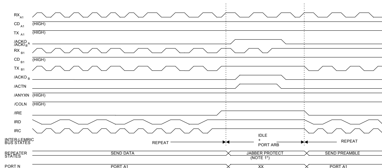
FIGURE 13. Jabber Protect
