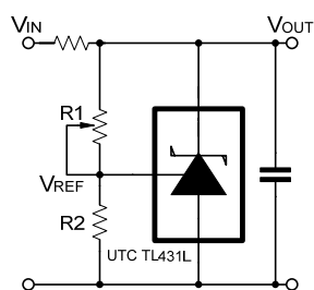
Shutdown Regulator
