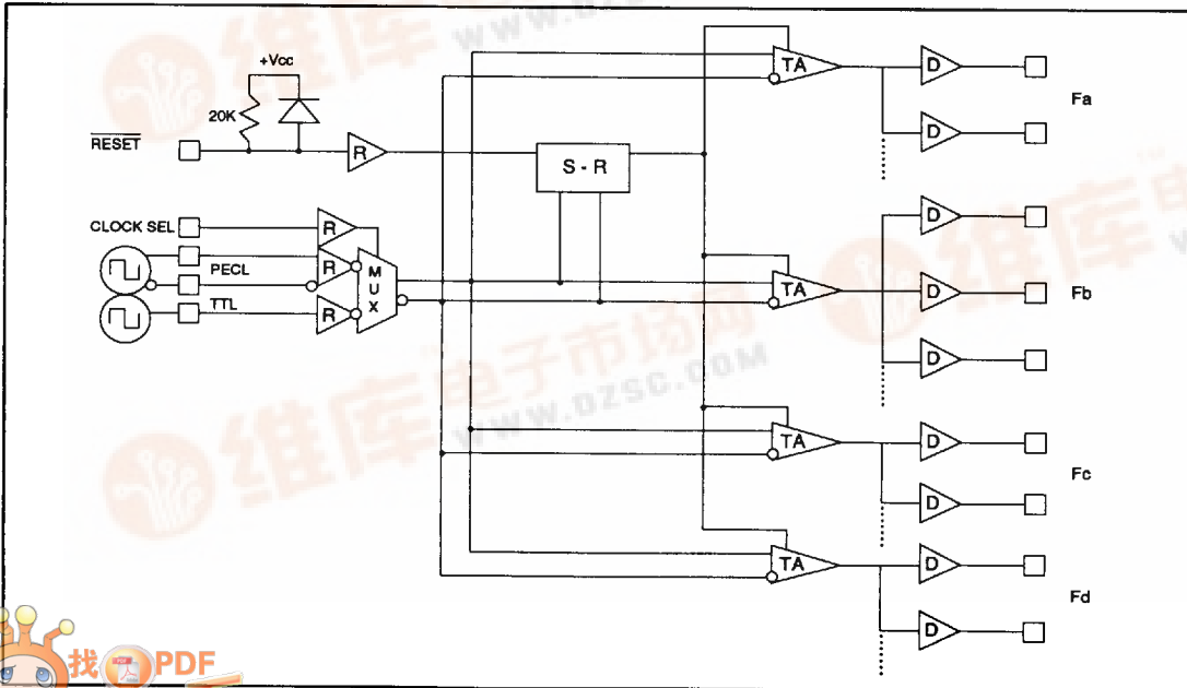
Figure 1. Logic Diagram
