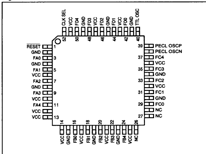
Figure 5. SC3508 Pinout
