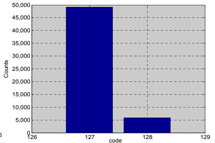
Figure 12. Noise Histogram
