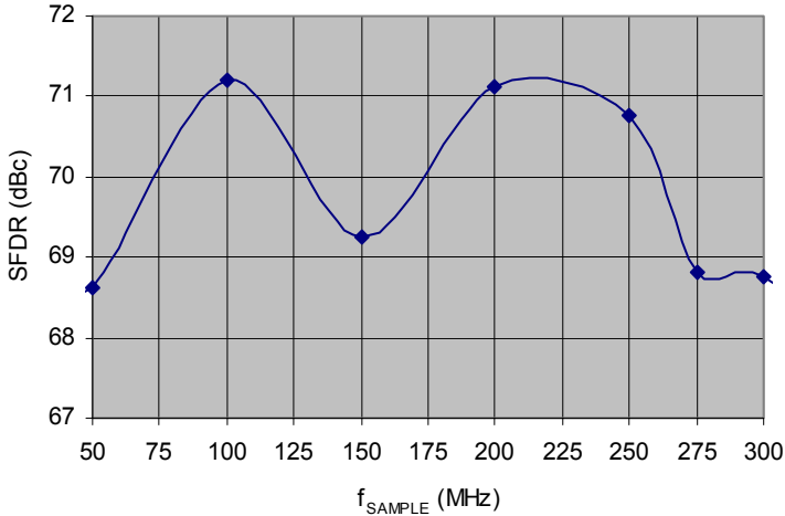
Figure 9. SFDR vs. f SAMPLE
