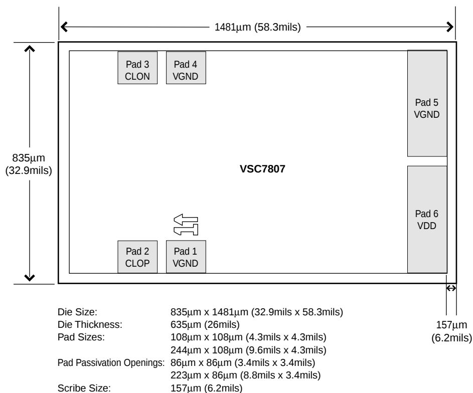
Figure 2: Pad Assignments
