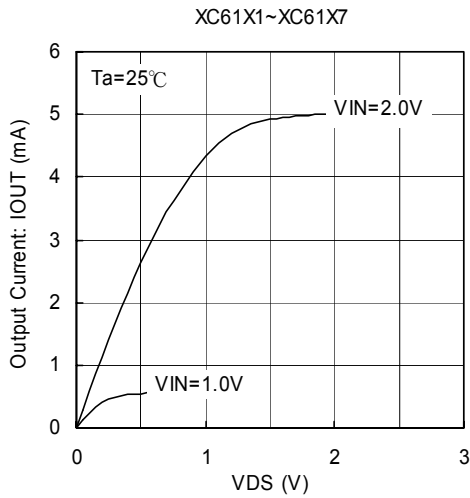
(4) N-ch Driver Output Current vs. VDS
