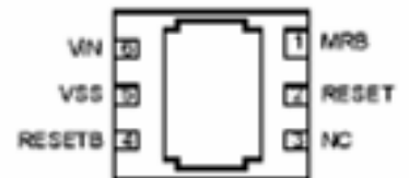
USP-6C (BOTTOM VIEW)
