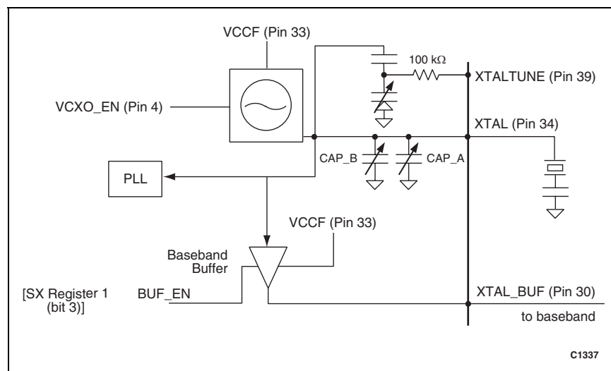
Figure 7. VCXO Block Diagram
