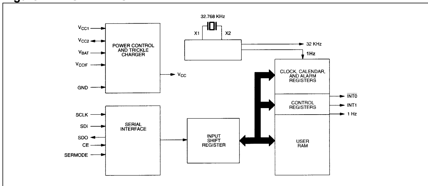
Figure 1. BLOCK DIAGRAM
