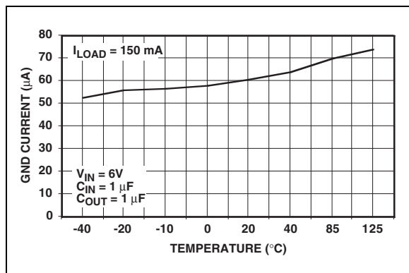
FIGURE 2-15: GND Current vs. Temperature ( I_{LOAD} = 150 mA ).
