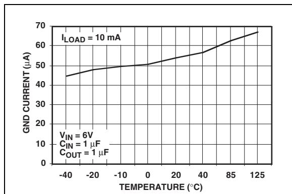
FIGURE 2-14: GND Current vs. Temperature ( I_{LOAD} = 10 mA ).
