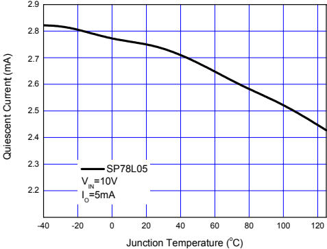
Figure 6. Quiescent Current vs. Junction Temperature
