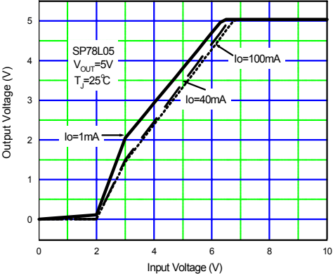
Figure 4. Dropout Characteristics
