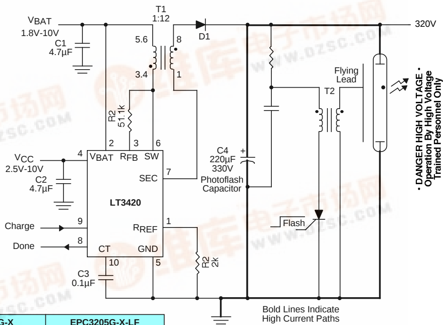
LT3420 320V Photoflash Capacitor Charging Circuit
