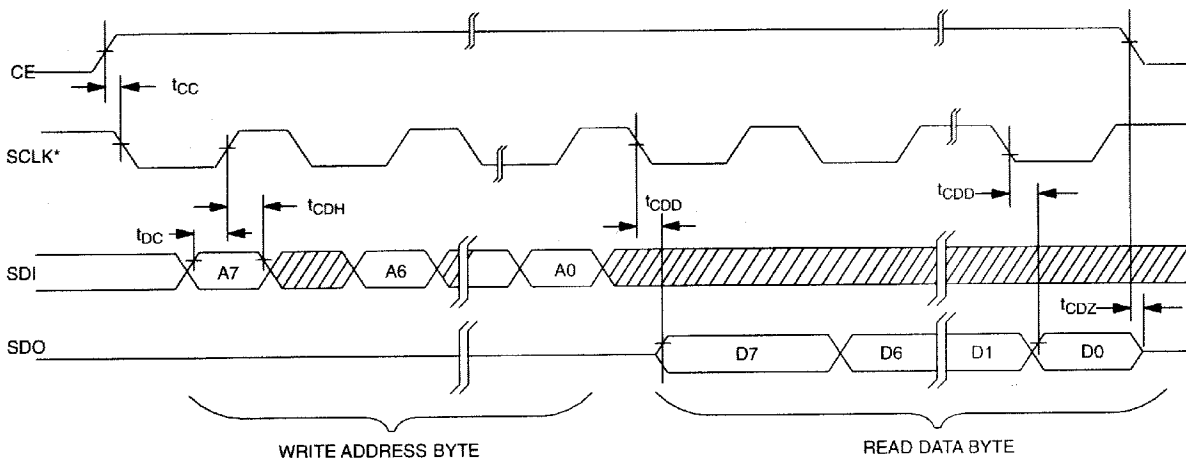
Figure 12. TIMING DIAGRAM: SPI READ DATA TRANSFER
