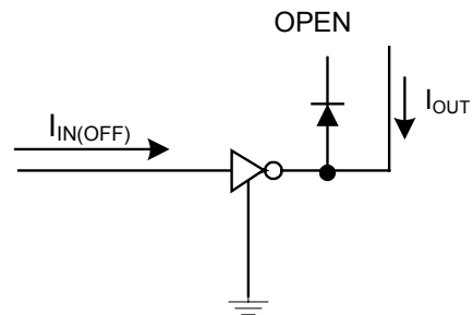
4. I_{IN(OFF)}
