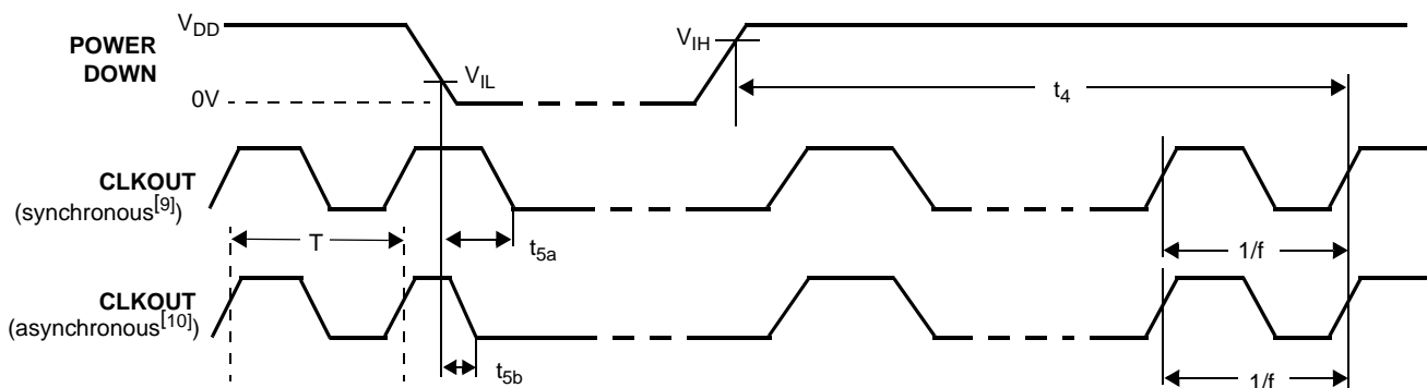
Figure 4. Power Down Timing (synchronous and asynchronous modes)
