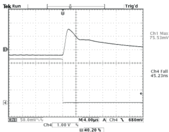
Figure 3 - Typical Transient Response (source) 12 A load Step di/dt = 300\text{ A}/\mu\text{s} Channel 1: Deviation on unit = 2.3%, Settling Time = 16 \mu\text{s} V_{in} = 5\text{ V} , V_{out} = 1.5\text{ V}
