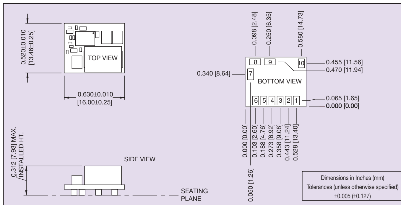
Figure 5 - Mechanical Drawing
