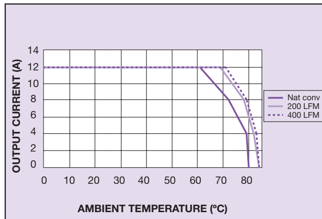
Figure 2 - Derating Curve V_{in} = 5\text{ V} , Output Voltage = 1.5 V (See Note A)
