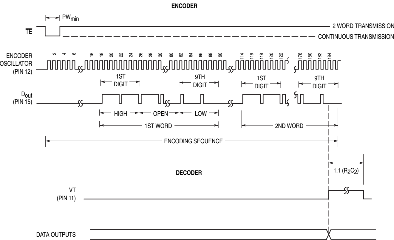
Figure 10. Timing Diagram
