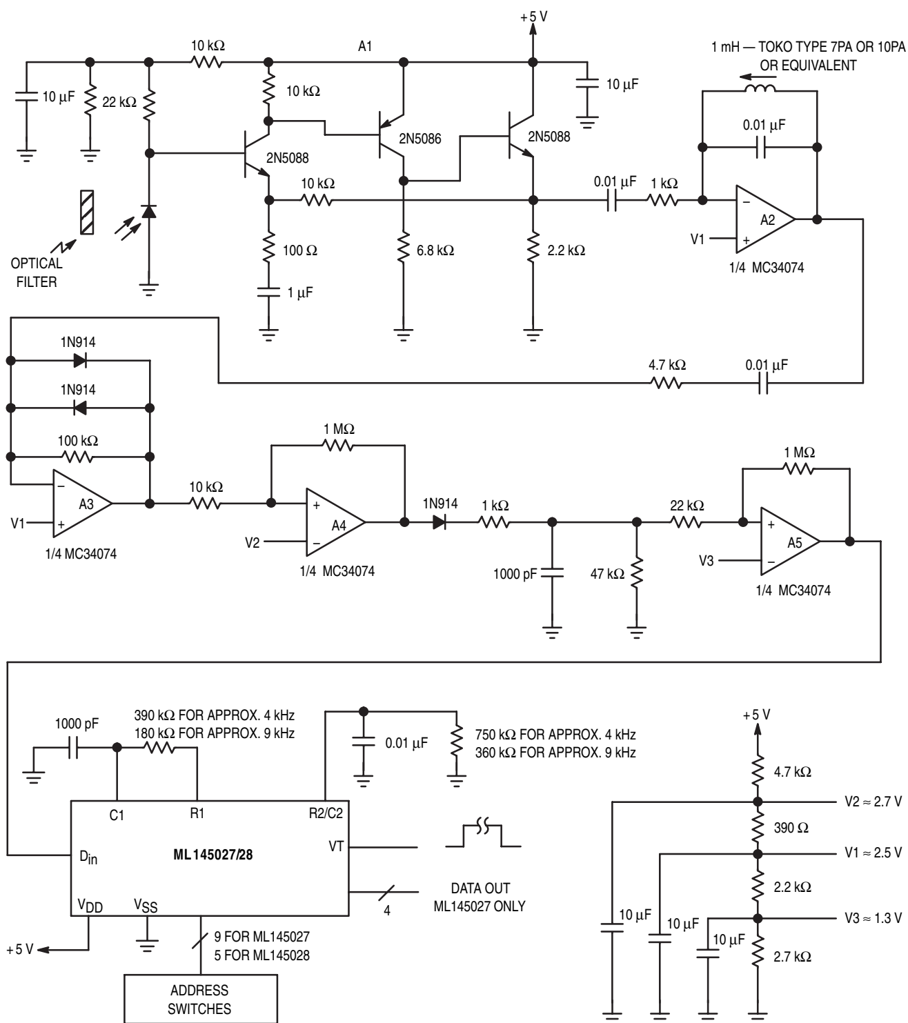
Figure 20. Infrared Receiver
