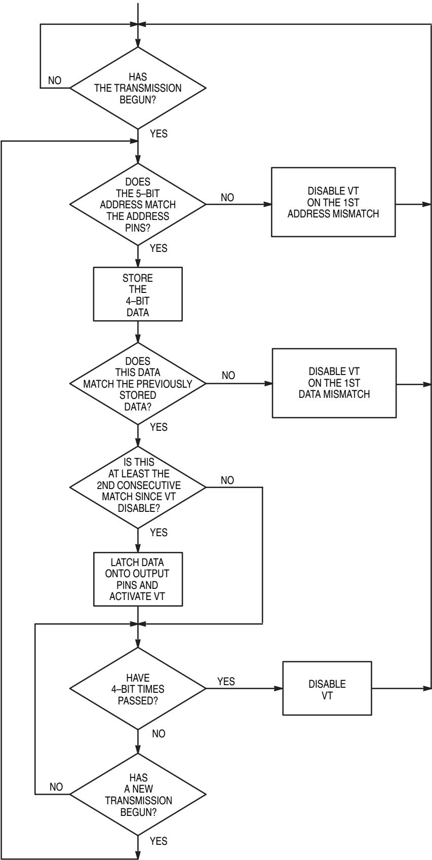
Figure 13. ML145027 Flowchart
