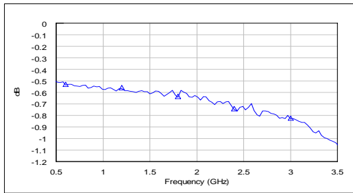
Insertion Loss
