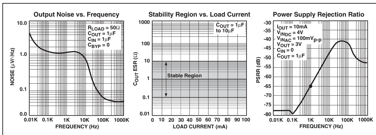
FIGURE 2-16: AC Characteristics.
