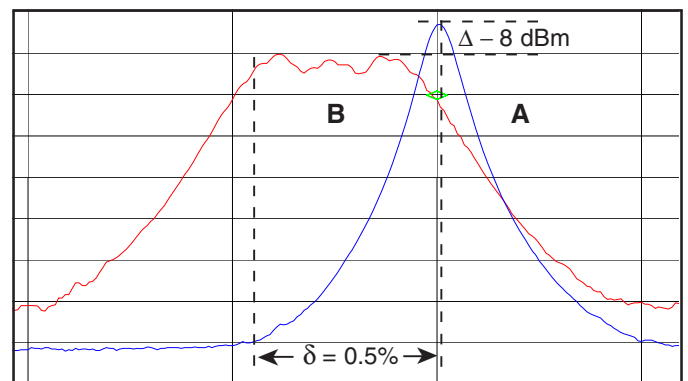
FIGURE 4B. 75MHz CLOCK OUTPUT IN FREQUENCY DOMAIN (A) SPREAD-SPECTRUM OFF (B) SPREAD-SPECTRUM ON
