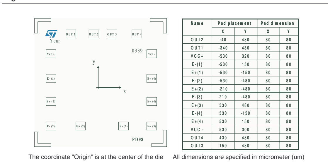
Figure 2. Pad locations
