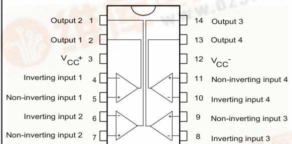
Pin connections (top view)
