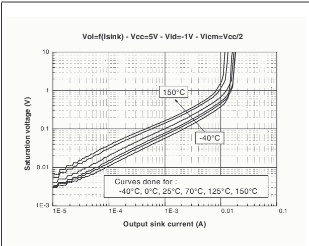
Figure 5. Output saturation voltage vs. output current (Vcc=5V)
