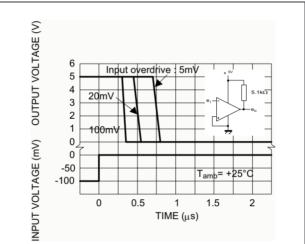
Figure 8. Response time for various input overdrives - negative transition
