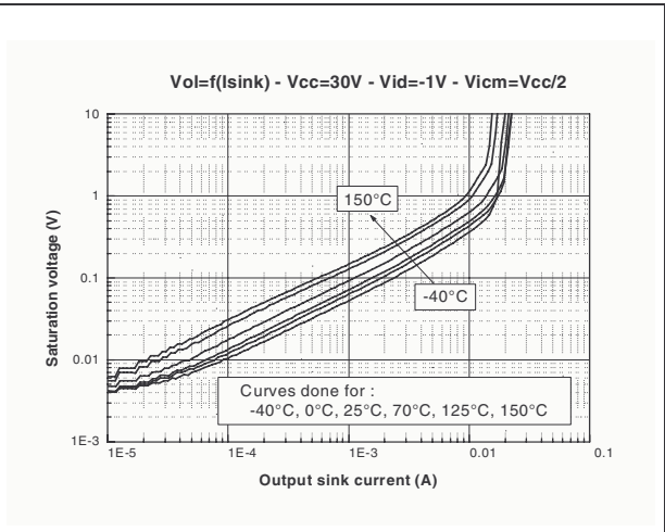
Figure 6. Output saturation voltage vs. output current (Vcc=30V)
