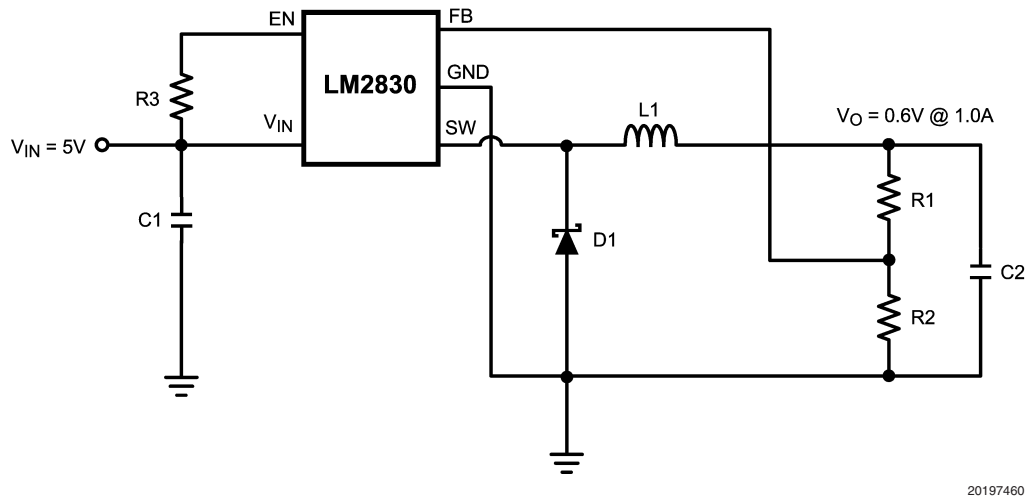
FIGURE 7. LM2830X (1.6MHz): V_{in} = 5V , V_o = 0.6V @ 1.0A
