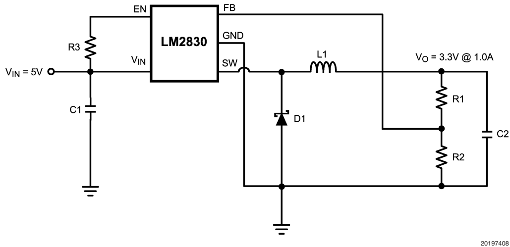
FIGURE 9. LM2830Z (3MHz): V_{in} = 5V , V_o = 3.3V @ 1.0A
