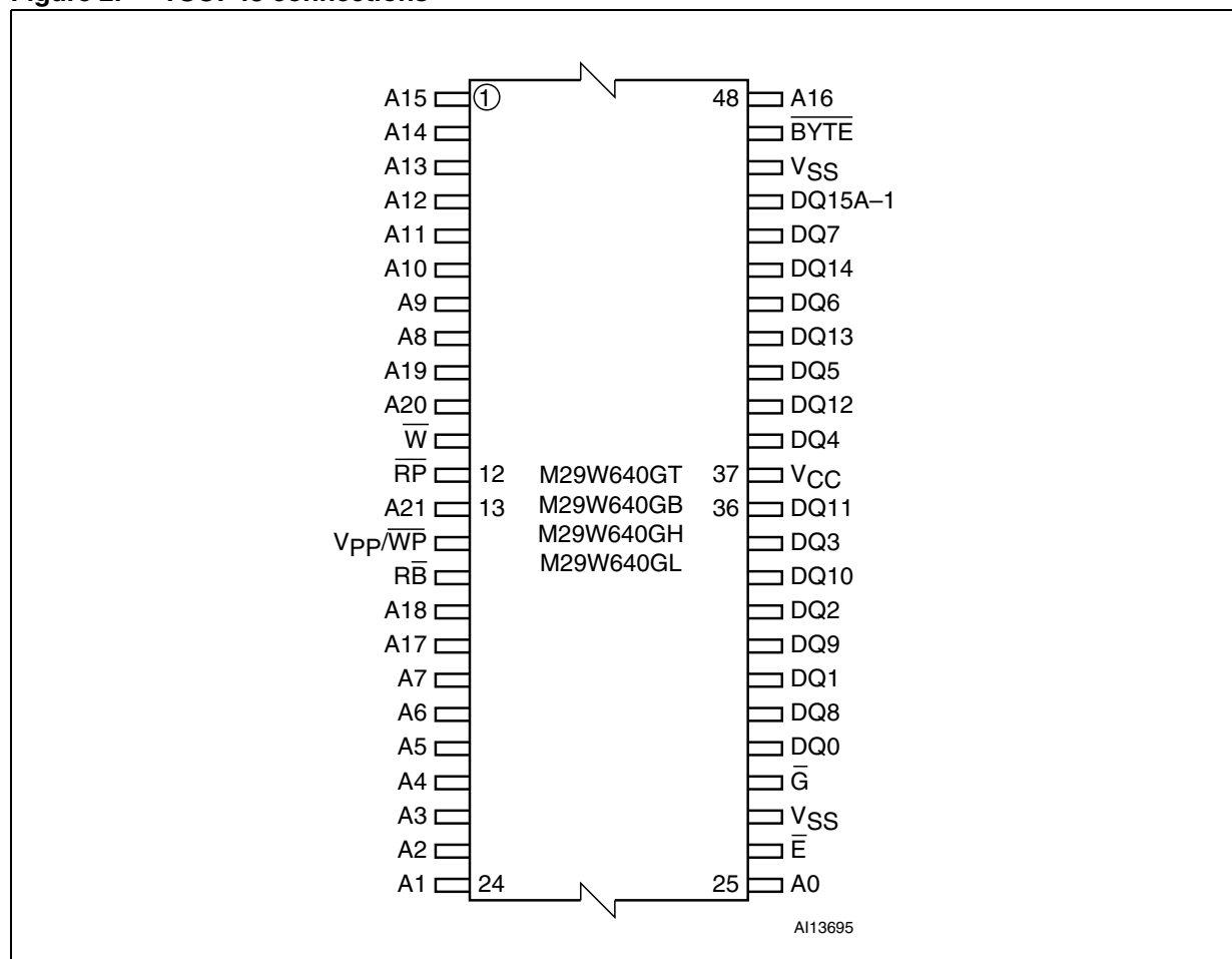
Figure 2. TSOP48 connections
