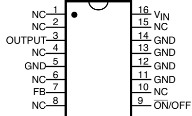
16-LEAD DIP (N)
