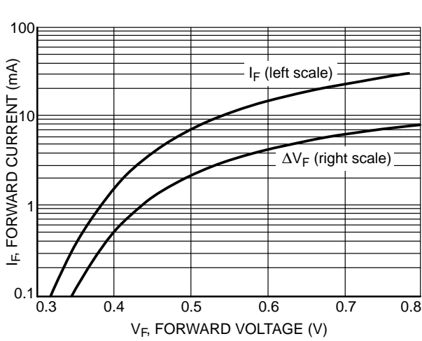
Figure 5. Typical V_F Match at Mixer Bias Levels
