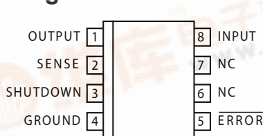
MIC29201-3.3BM (SOIC-8)
