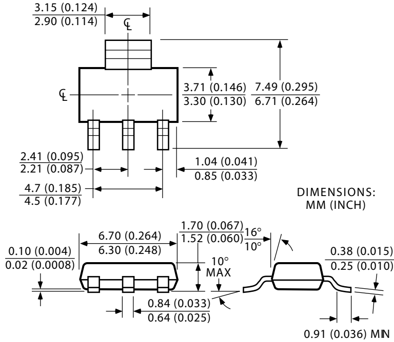
SOT-223 (S)
