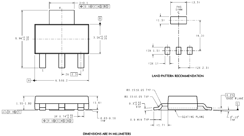
3-Lead SOT-223 Package NS Package Number MP04A
