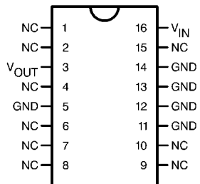
Top View See NS Package Number J16A
