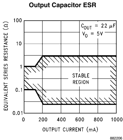
FIGURE 1. ESR Limits
