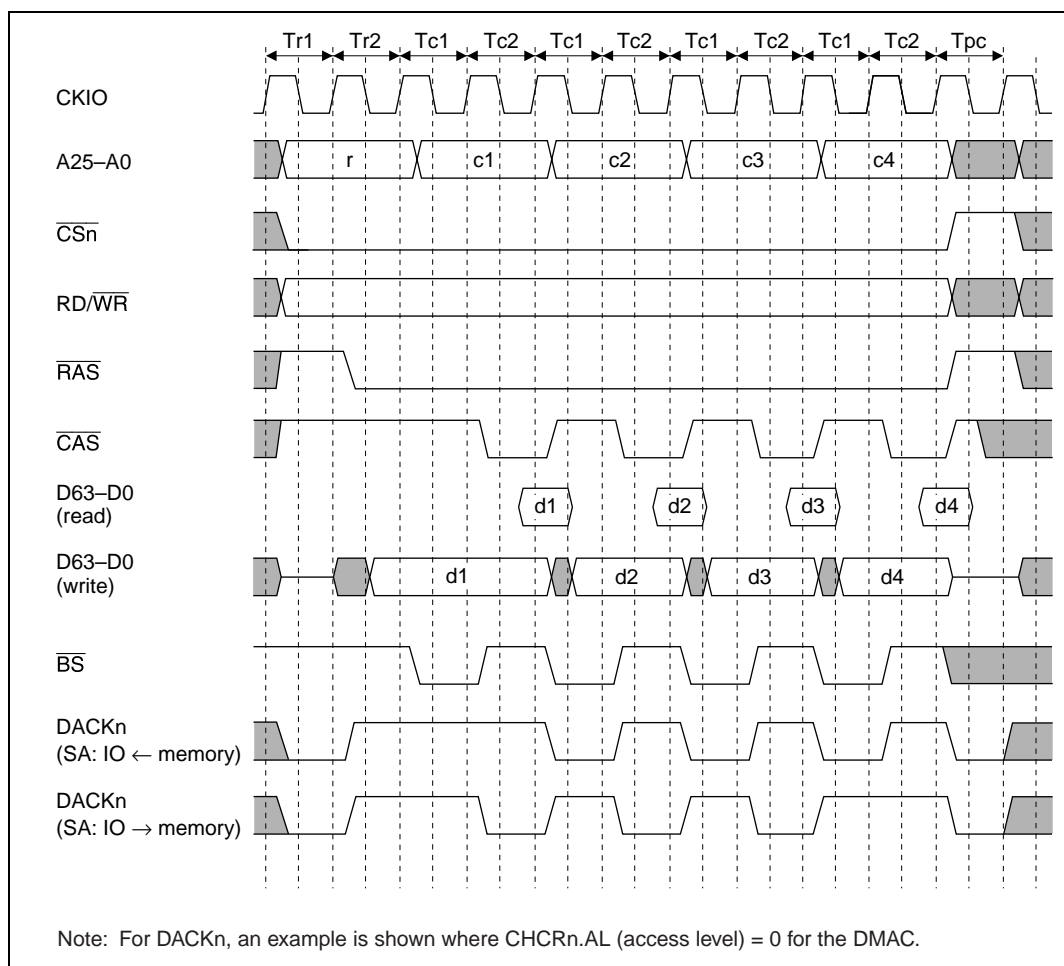
Figure 13.19 DRAM Burst Access Timing
