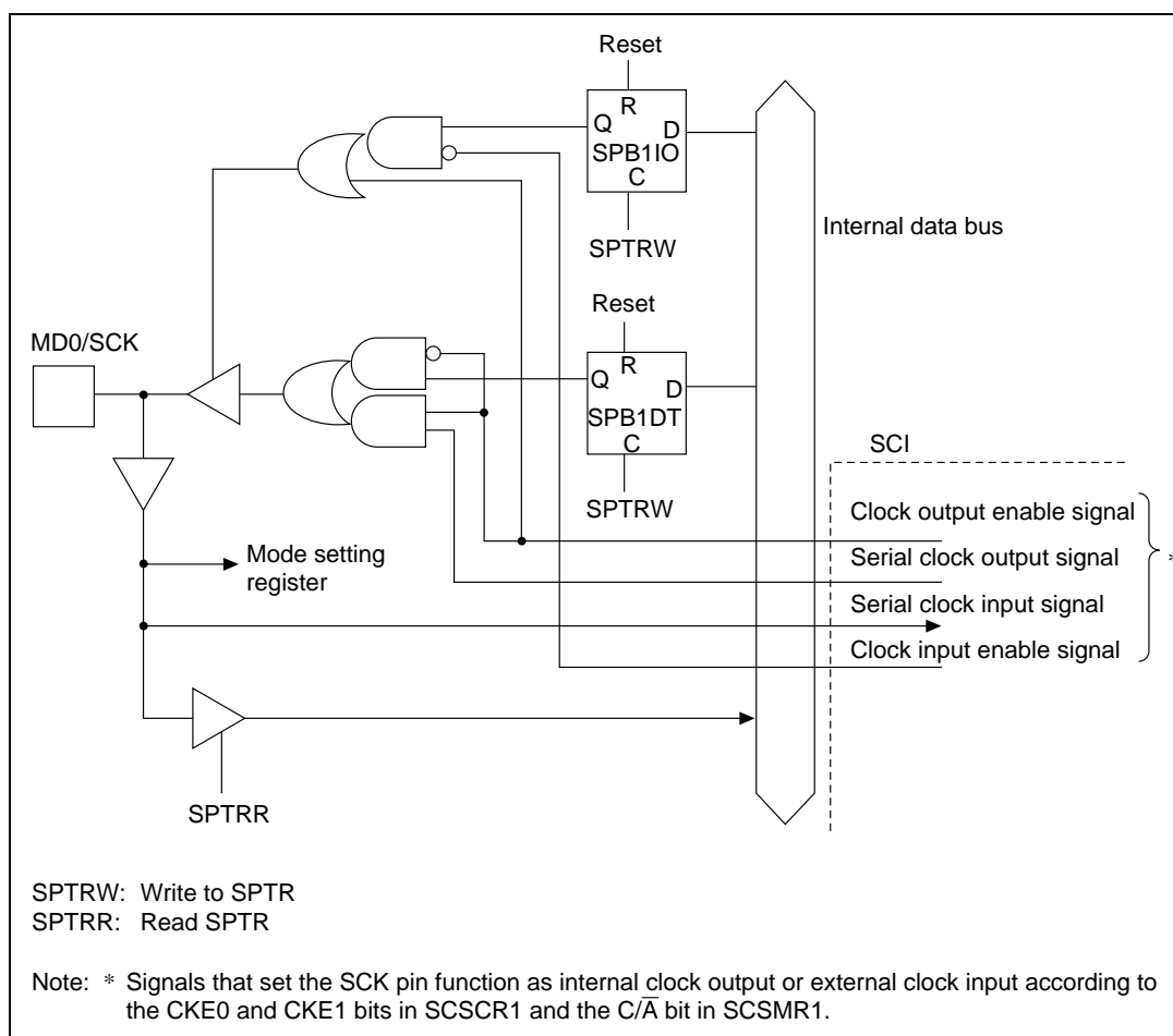
Figure 18.3 MD0/SCK Pin
