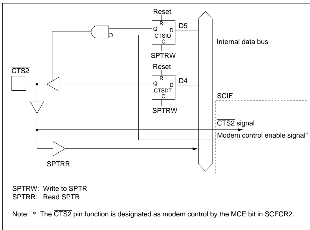
Figure 16.3 \overline{\text{CTS2}} Pin
