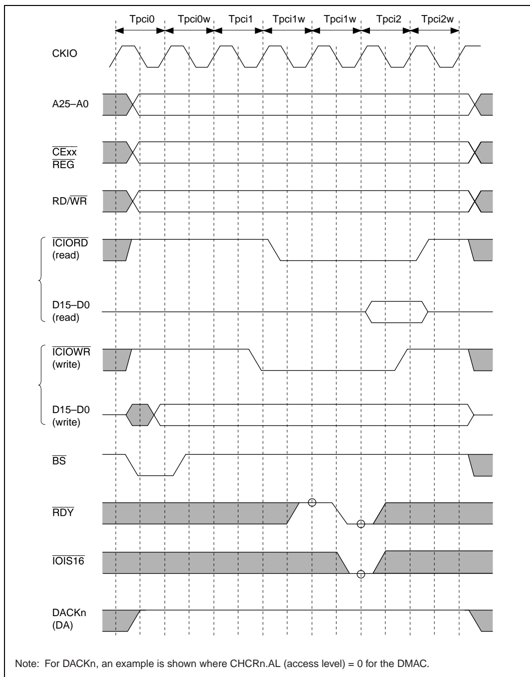
Figure 13.54 Wait Timing for PCMCIA I/O Card Interface
