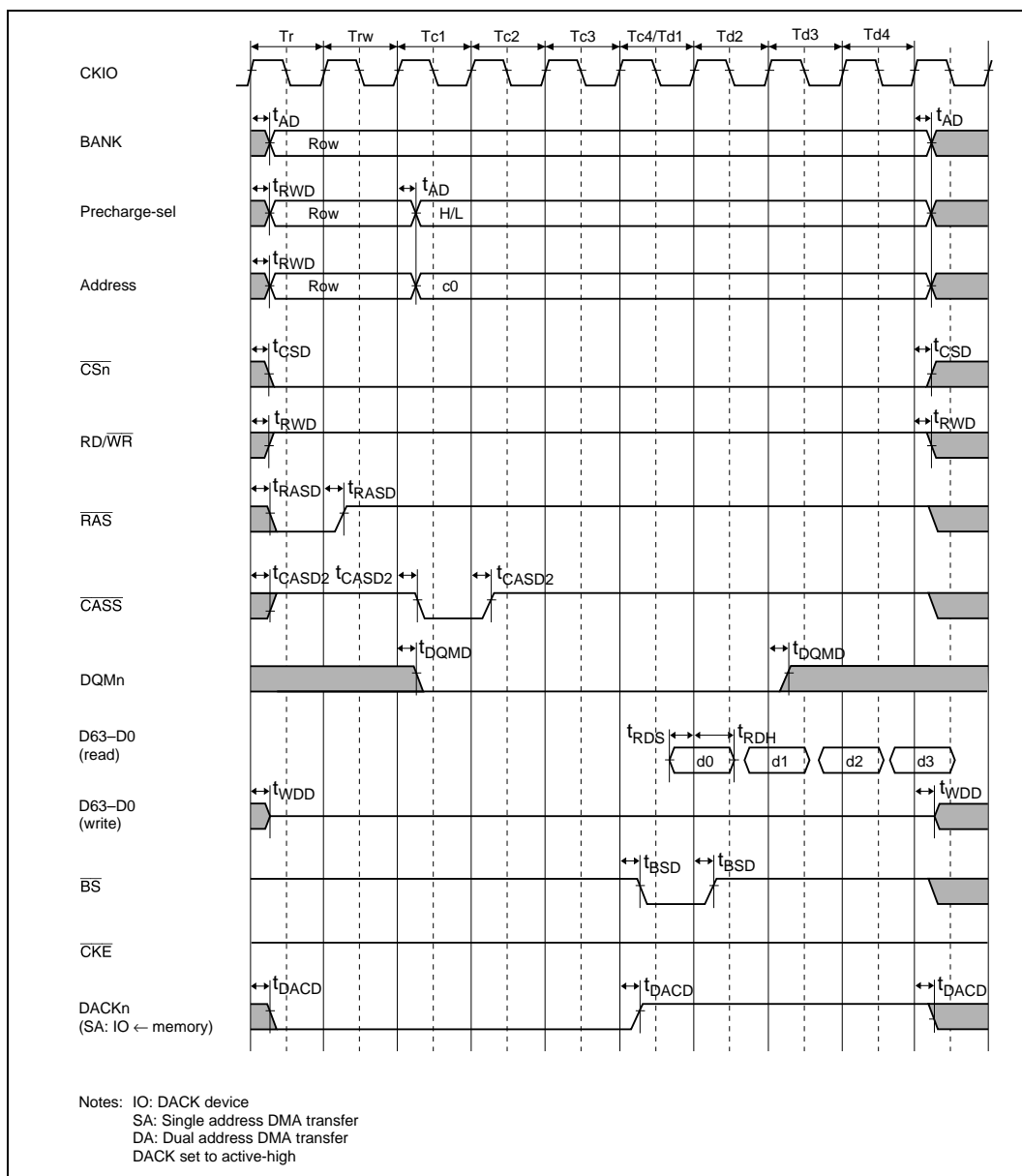
Figure 22.25 Synchronous DRAM Normal Read Bus Cycle: ACT + READ Commands, Burst (RCD[1:0] = 01, CAS Latency = 3)
