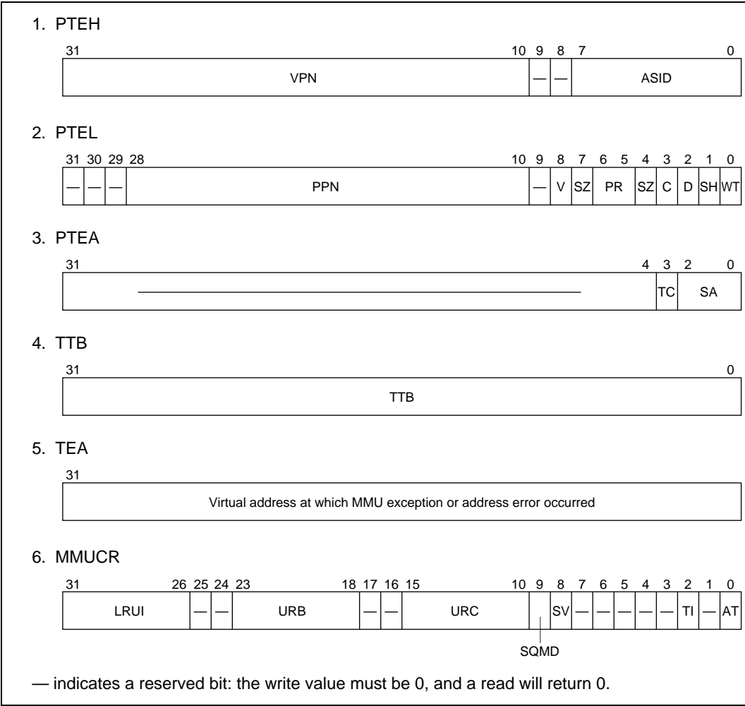
Figure 3.2 MMU-Related Registers
