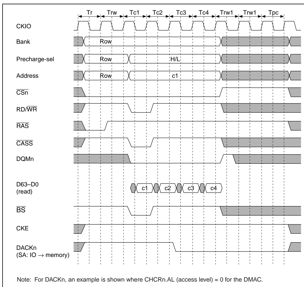
Figure 13.30 Basic Timing for Synchronous DRAM Burst Write
