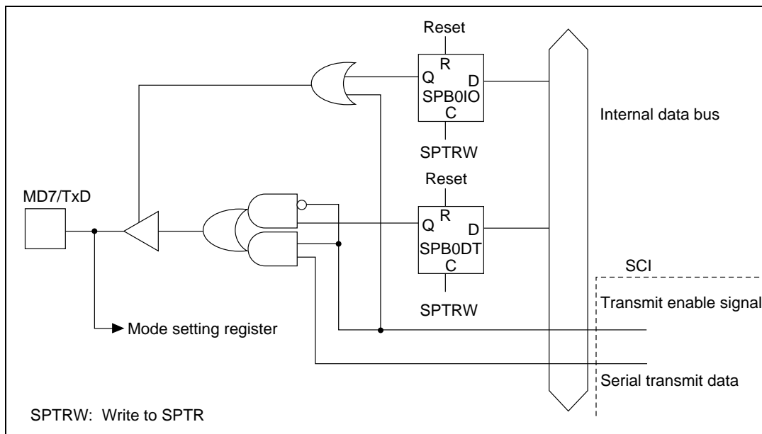
Figure 15.3 MD7/TxD Pin
