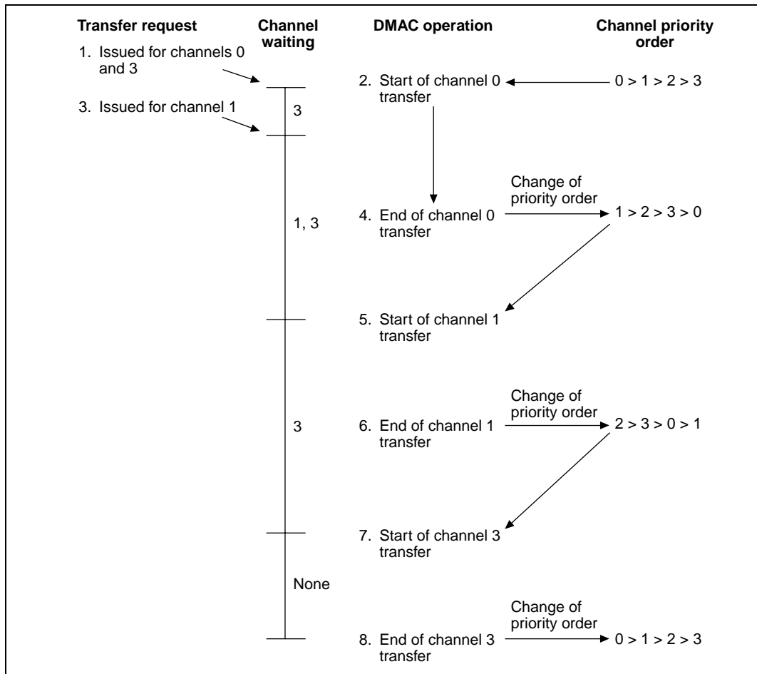
Figure 14.4 Example of Changes in Priority Order in Round Robin Mode
