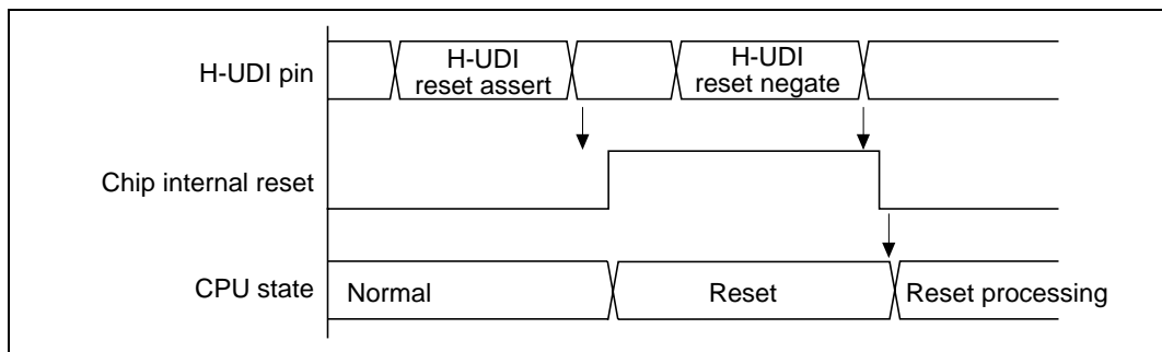
Figure 21.3 H-UDI Reset
