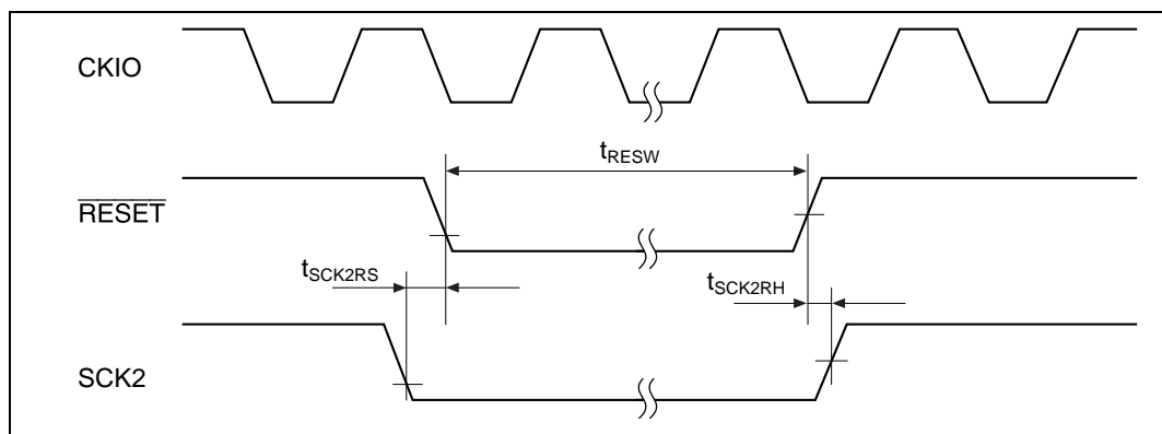
Figure 22.11 Manual Reset Input Timing
