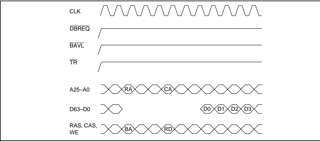
Figure 14.35 Read from Synchronous DRAM Precharge Bank
