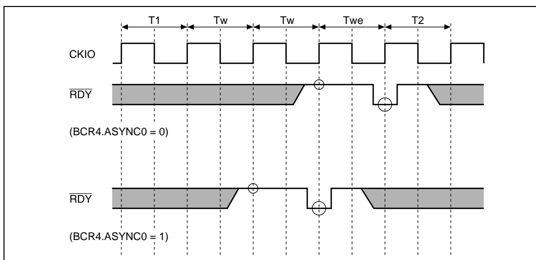
Figure 13.4 Example of \overline{RDY} Sampling Timing at which BCR4 is Set (Two Wait Cycles are Inserted by WCR2)
