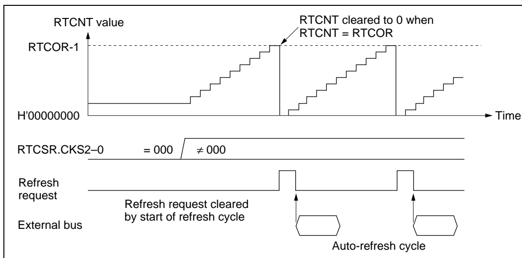
Figure 13.39 Auto-Refresh Operation
