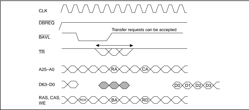
Figure 14.36 Read from Synchronous DRAM Non-Precharge Bank (Row Miss)
