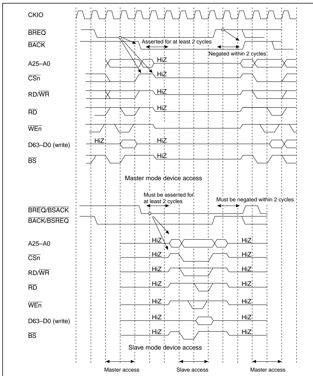
Figure 13.78 Arbitration Sequence
