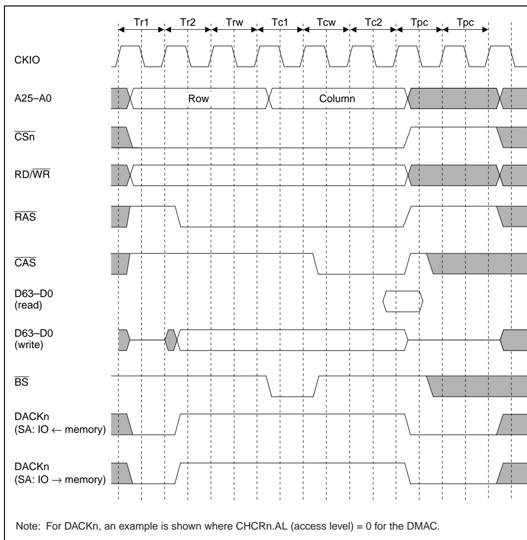
Figure 13.18 DRAM Wait State Timing
