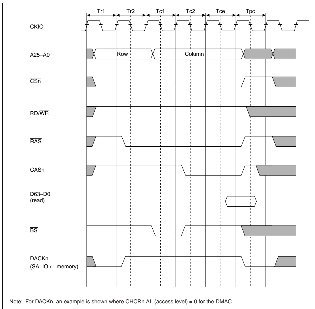
Figure 13.20 DRAM Bus Cycle (EDO Mode, RCD = 0, AnW = 0, TPC = 1)
