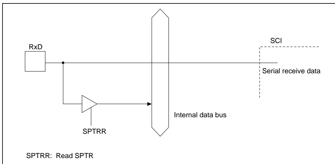
Figure 15.4 RxD Pin
