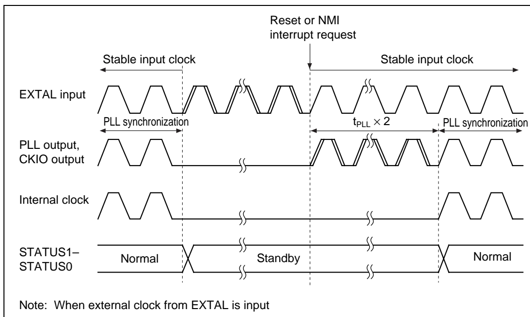
Figure 22.9 PLL Synchronization Settling Time in Case of \overline{\text{RESET}} or NMI Interrupt
