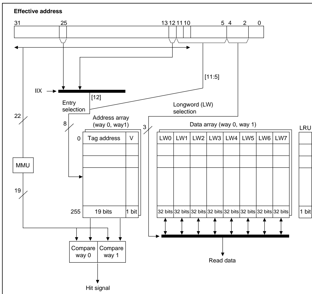
Figure 4.7 Configuration of Instruction Cache (SH7750R)
