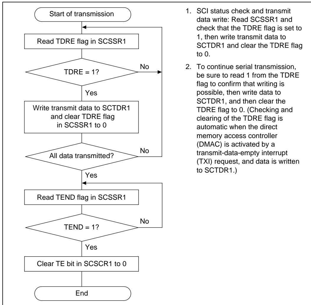
Figure 15.19 Sample Serial Transmission Flowchart
