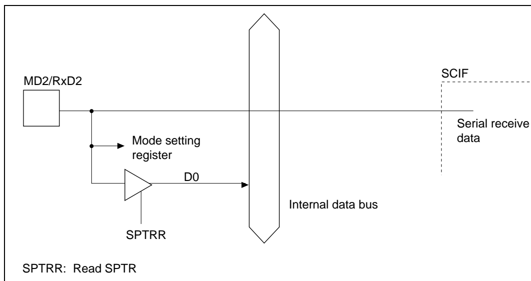
Figure 16.5 MD2/RxD2 Pin
