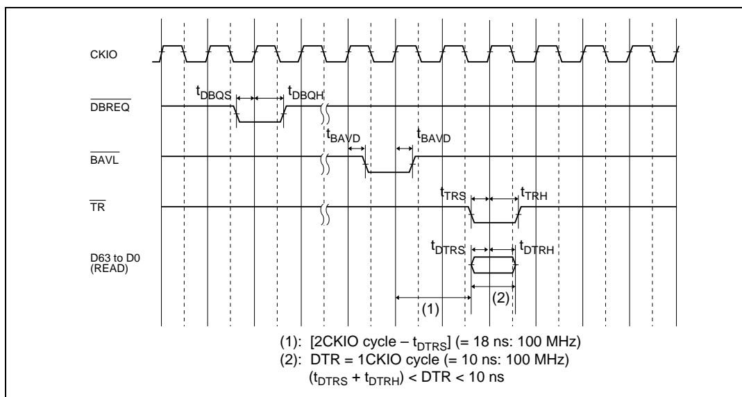
Figure 22.66(b) DBREQ/TR Input Timing and BAVL Output Timing
