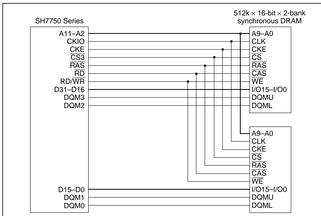
Figure 13.27 Example of 32-Bit Data Width Synchronous DRAM Connection (Area 3)
