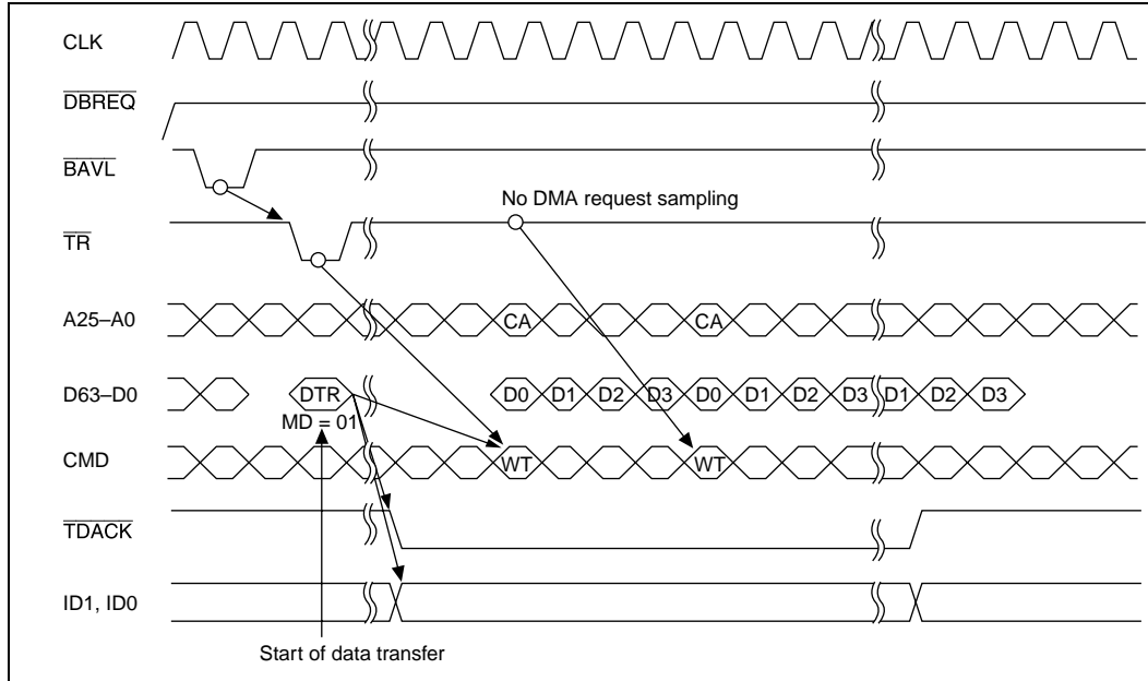
Figure 14.43 Single Address Mode/Burst Mode/Edge Detection/ External Device → External Bus Data Transfer
