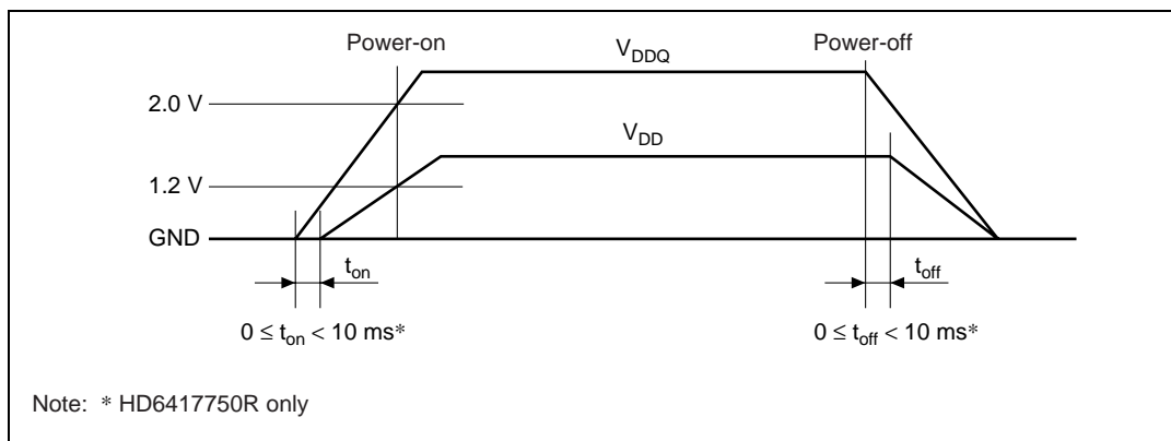
Figure H.1 Power-On and Power-Off Procedures
