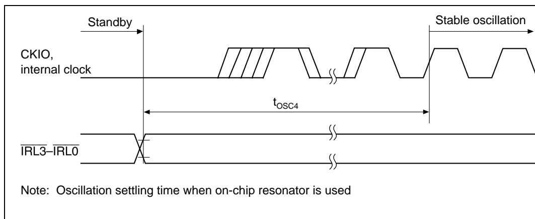
Figure 22.8 Standby Return Oscillation Settling Time (Return by \overline{\text{IRL3}}\text{--}\overline{\text{IRL0}} )
