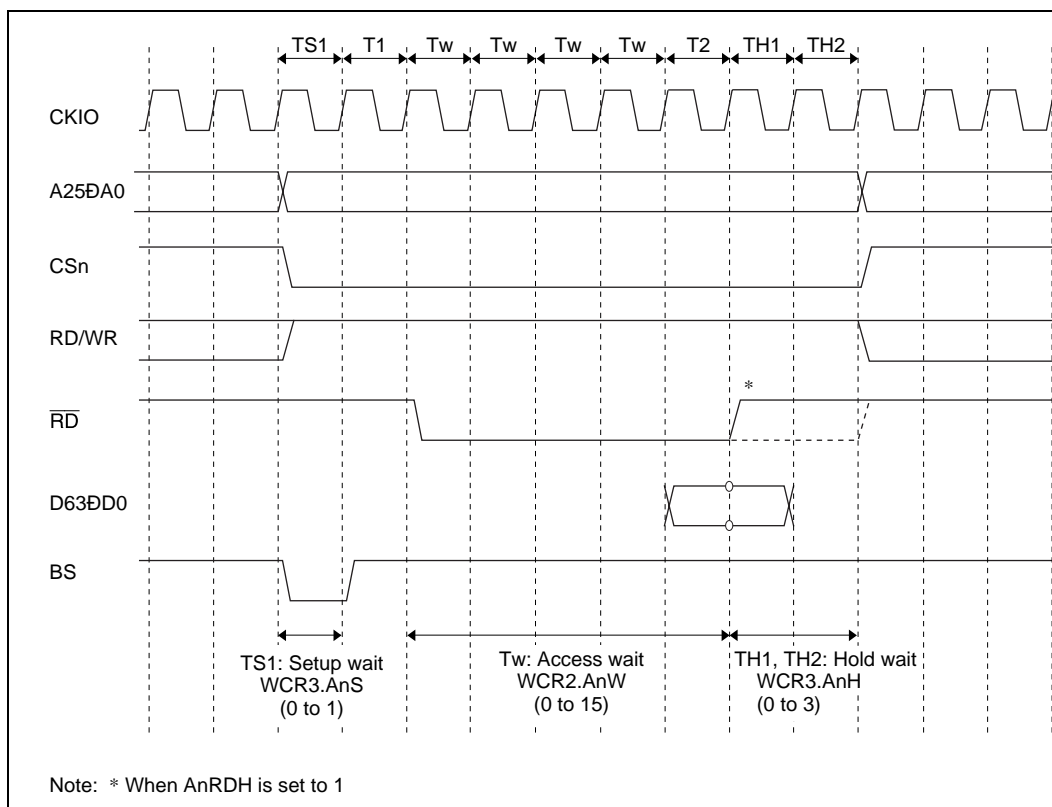
Figure 13.13 SRAM Interface Read-Strobe Negate Timing (AnS = 1, AnW = 4, AnH = 2)
