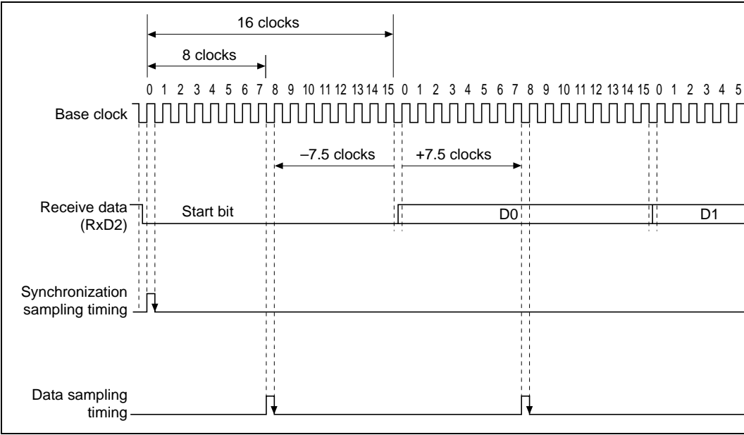
Figure 16.13 Receive Data Sampling Timing in Asynchronous Mode
