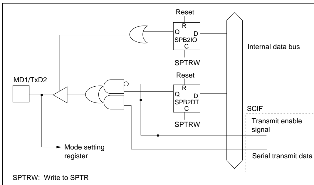
Figure 18.6 MD1/TxD2 Pin
