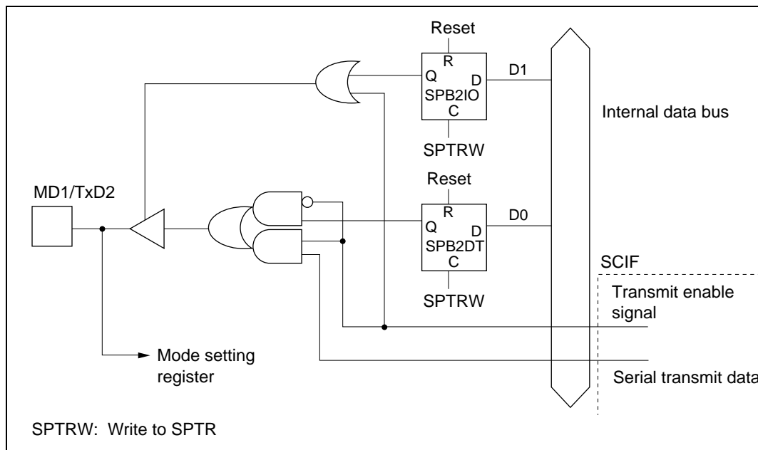
Figure 16.4 MD1/TxD2 Pin
