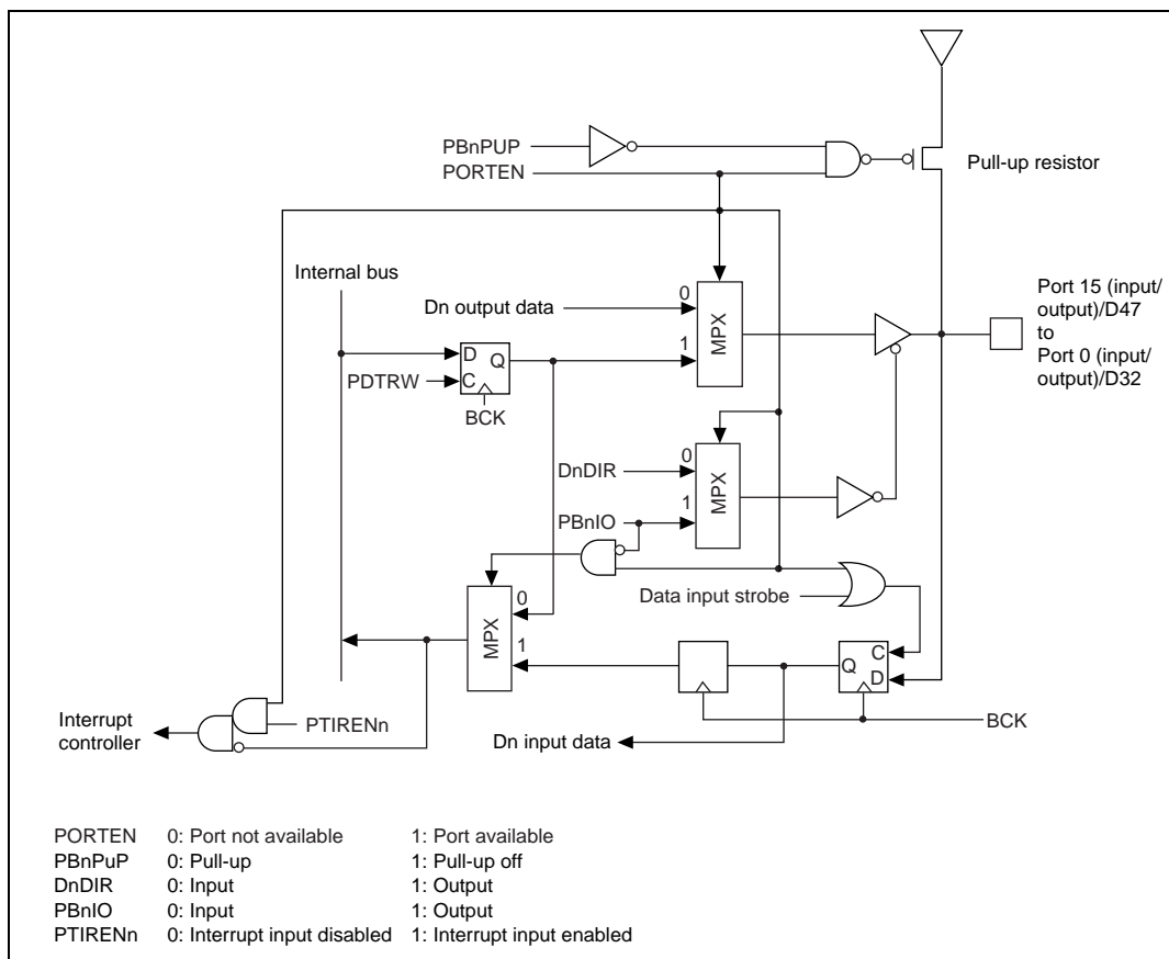
Figure 18.1 16-Bit Port
