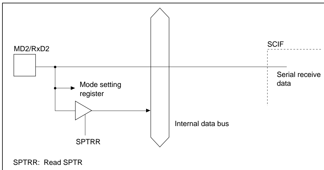
Figure 18.7 MD2/RxD2 Pin
