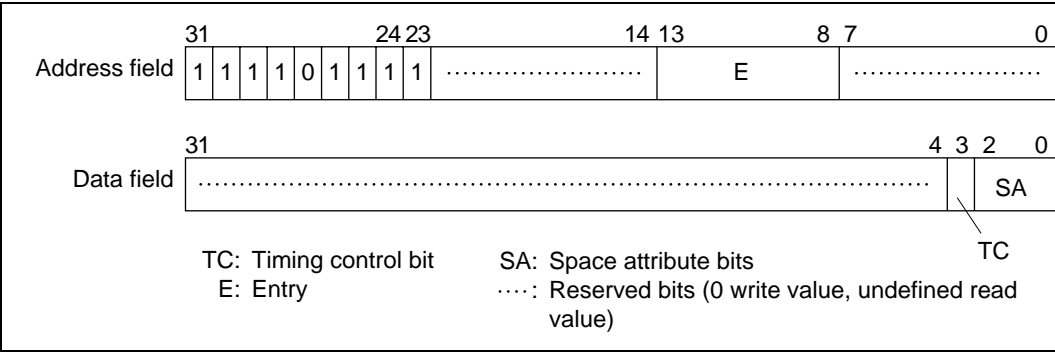
Figure 3.18 Memory-Mapped UTLB Data Array 2
