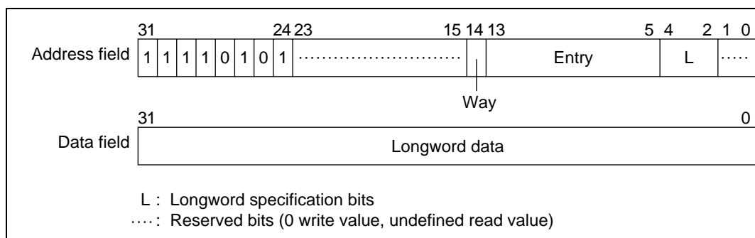
Figure 4.15 Memory-Mapped OC Data Array
