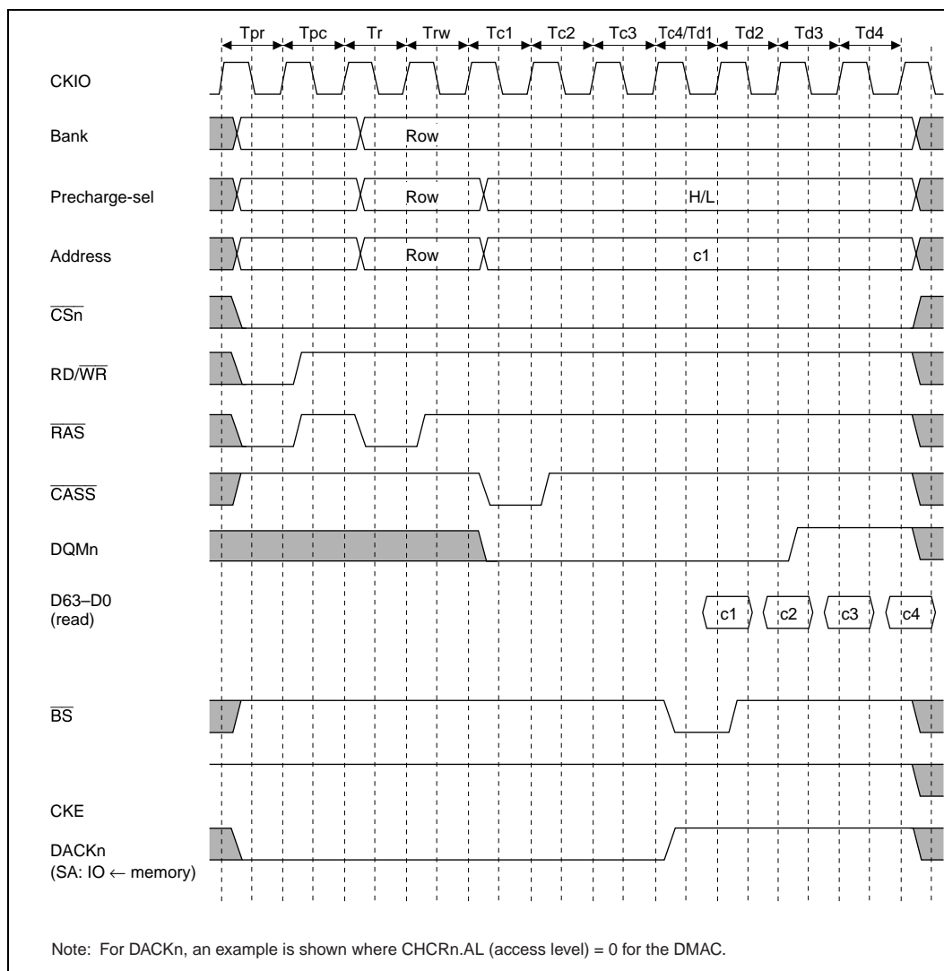
Figure 13.34 Burst Read Timing (RAS Down, Different Row Addresses)
