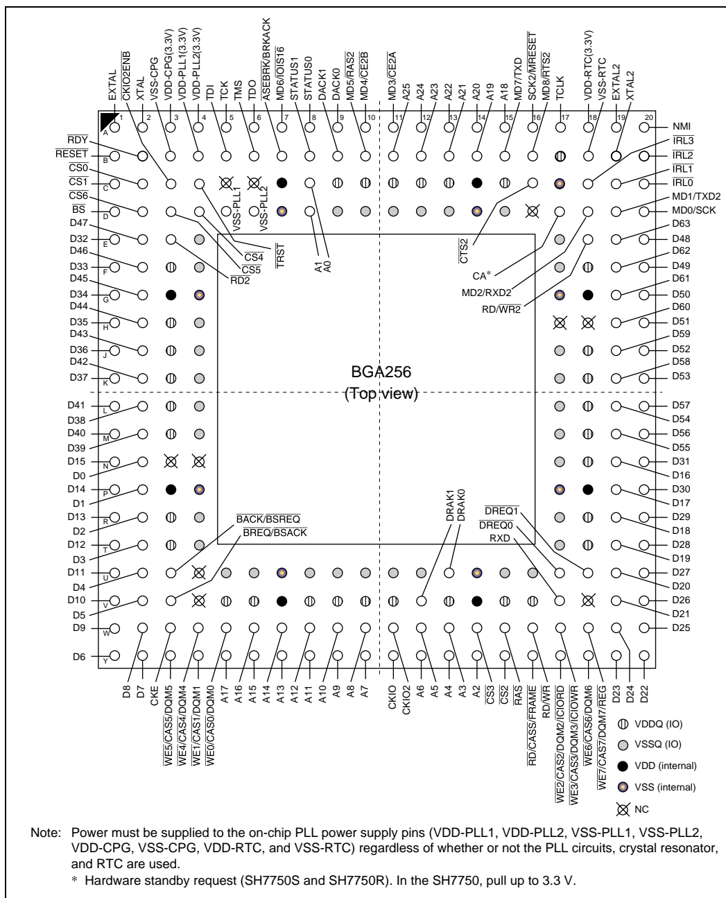
Figure 1.2 Pin Arrangement (256-Pin BGA)
