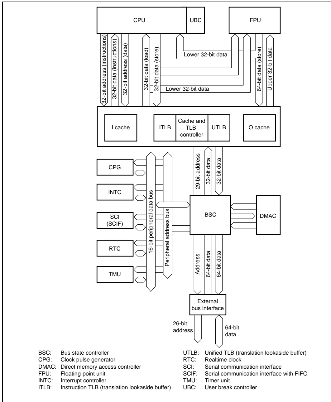
Figure 1.1 Block Diagram of SH7750 Series Functions
