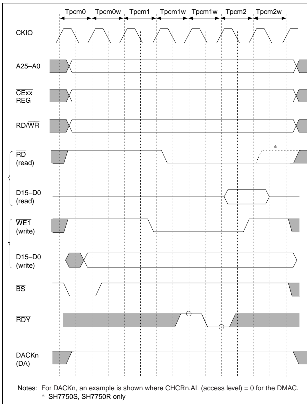
Figure 13.51 Wait Timing for PCMCIA Memory Card Interface
