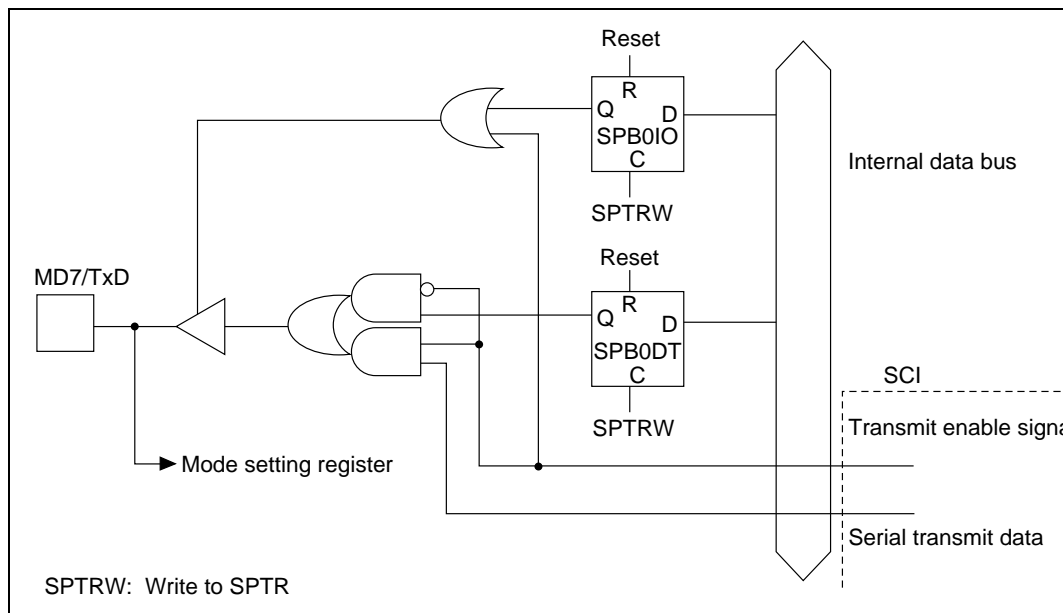
Figure 18.4 MD7/TxD Pin
