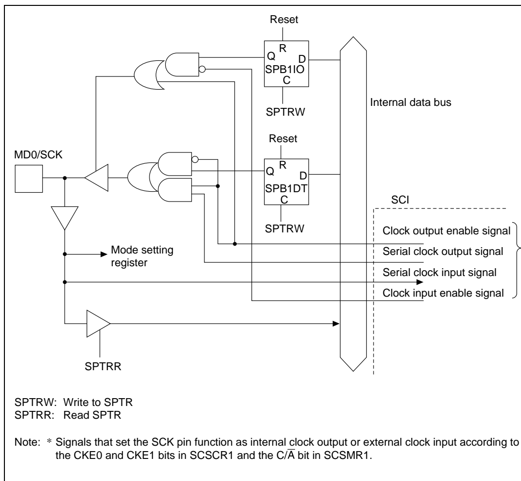
Figure 15.2 MD0/SCK Pin
