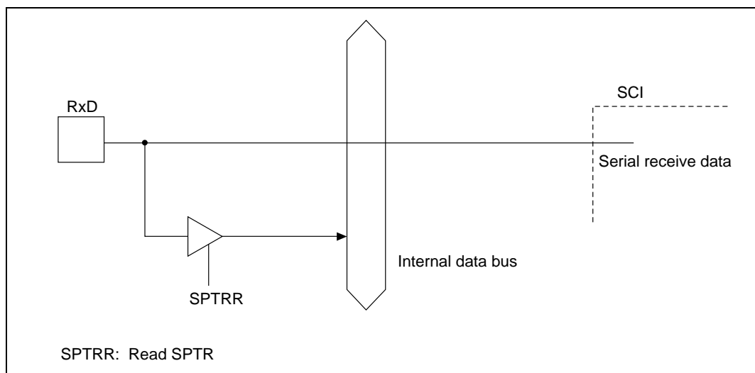
Figure 18.5 RxD Pin
