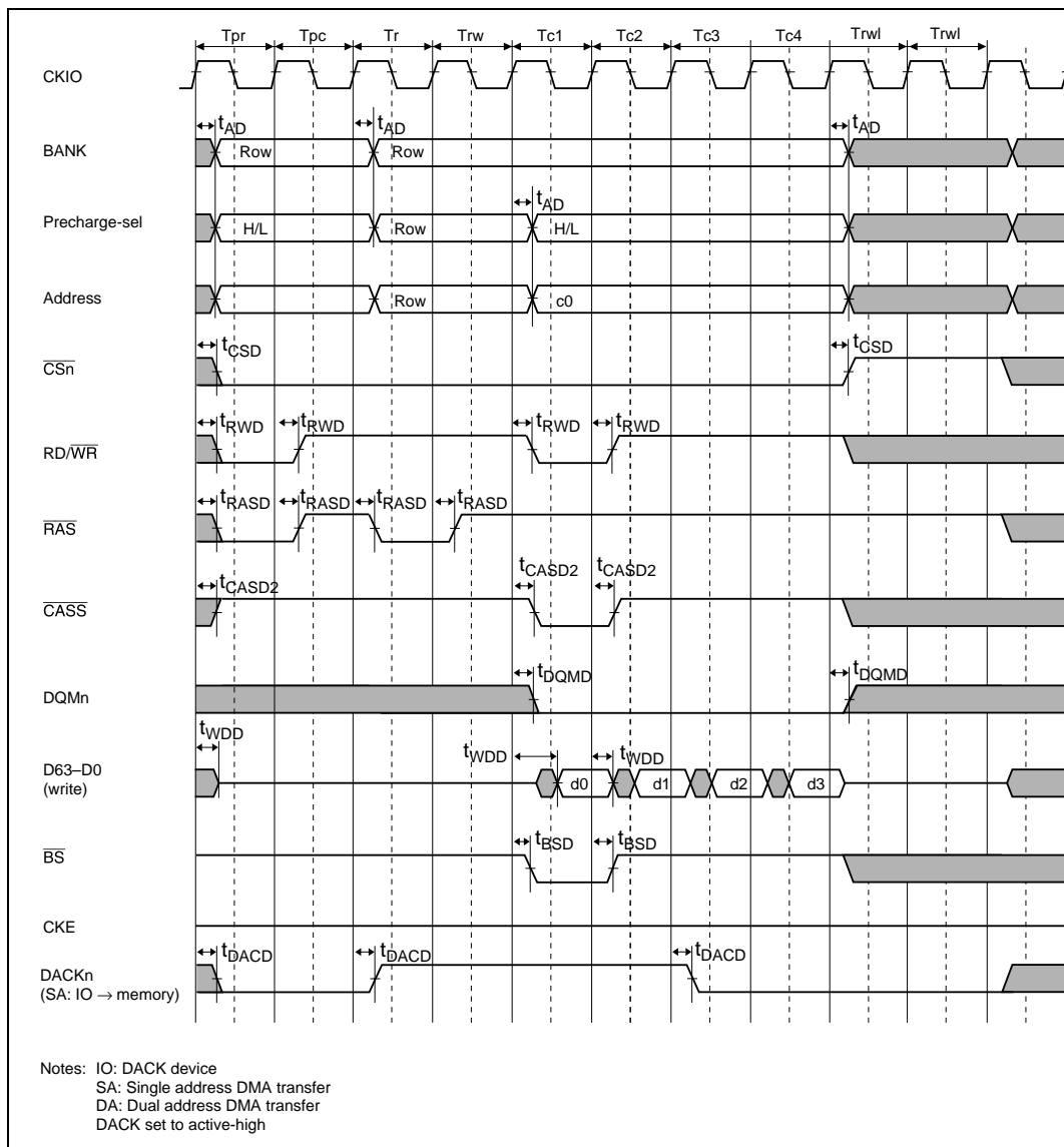
Figure 22.31 Synchronous DRAM Normal Write Bus Cycle: PRE + ACT + WRITE Commands, Burst (RCD[1:0] = 01, TPC[2:0] = 001, TRWL[2:0] = 010)
