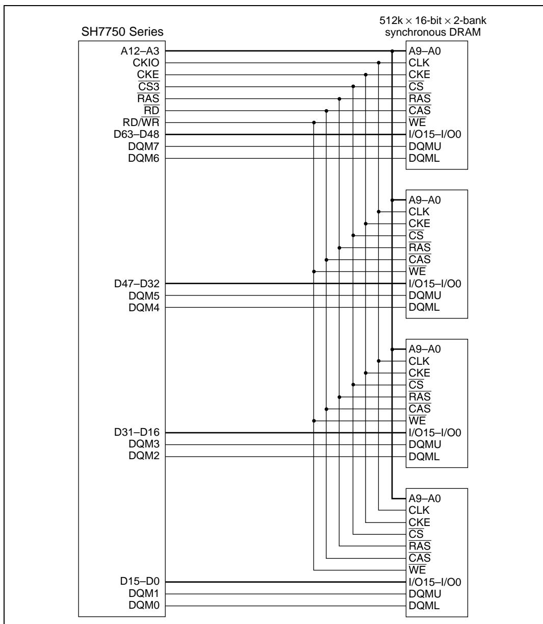
Figure 13.26 Example of 64-Bit Data Width Synchronous DRAM Connection (Area 3)
