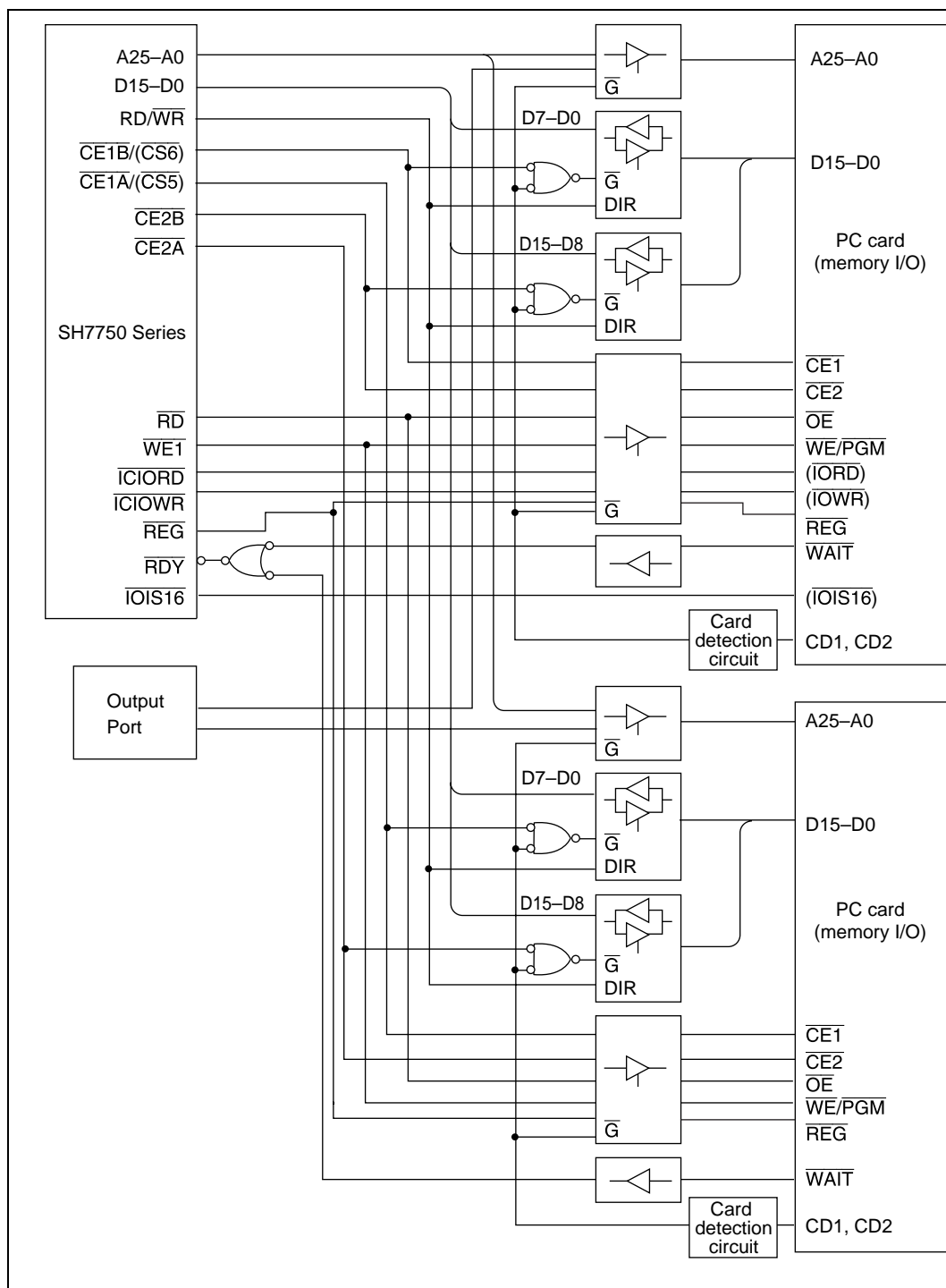
Figure 13.49 Example of PCMCIA Interface
