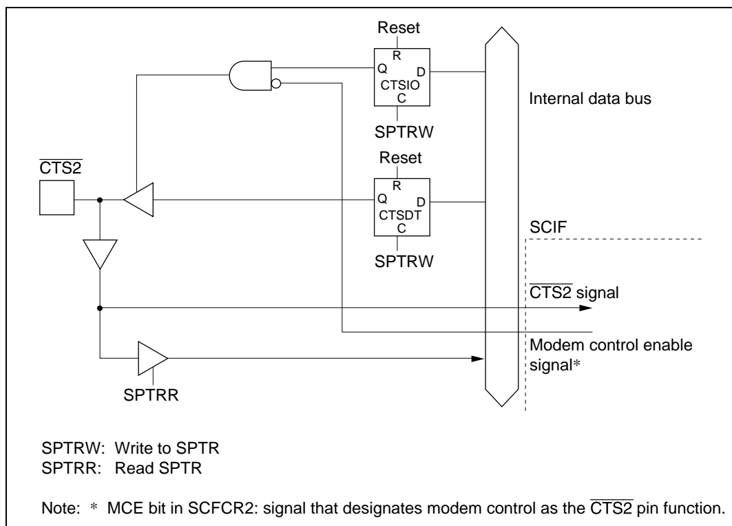
Figure 18.8 \overline{\text{CTS2}} Pin
