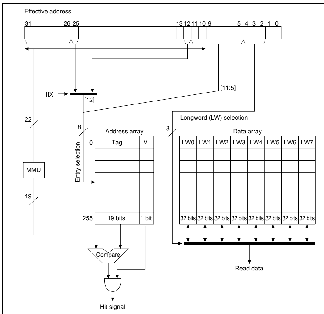
Figure 4.6 Configuration of Instruction Cache (SH7750, SH7750S)
