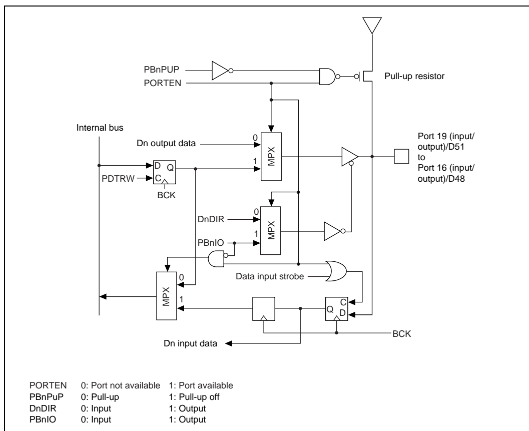
Figure 18.2 4-Bit Port
