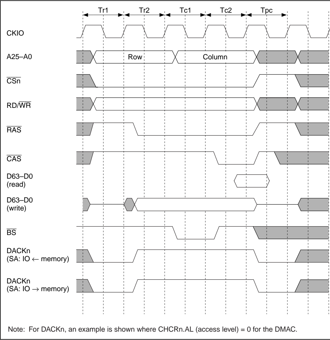
Figure 13.17 Basic DRAM Access Timing
