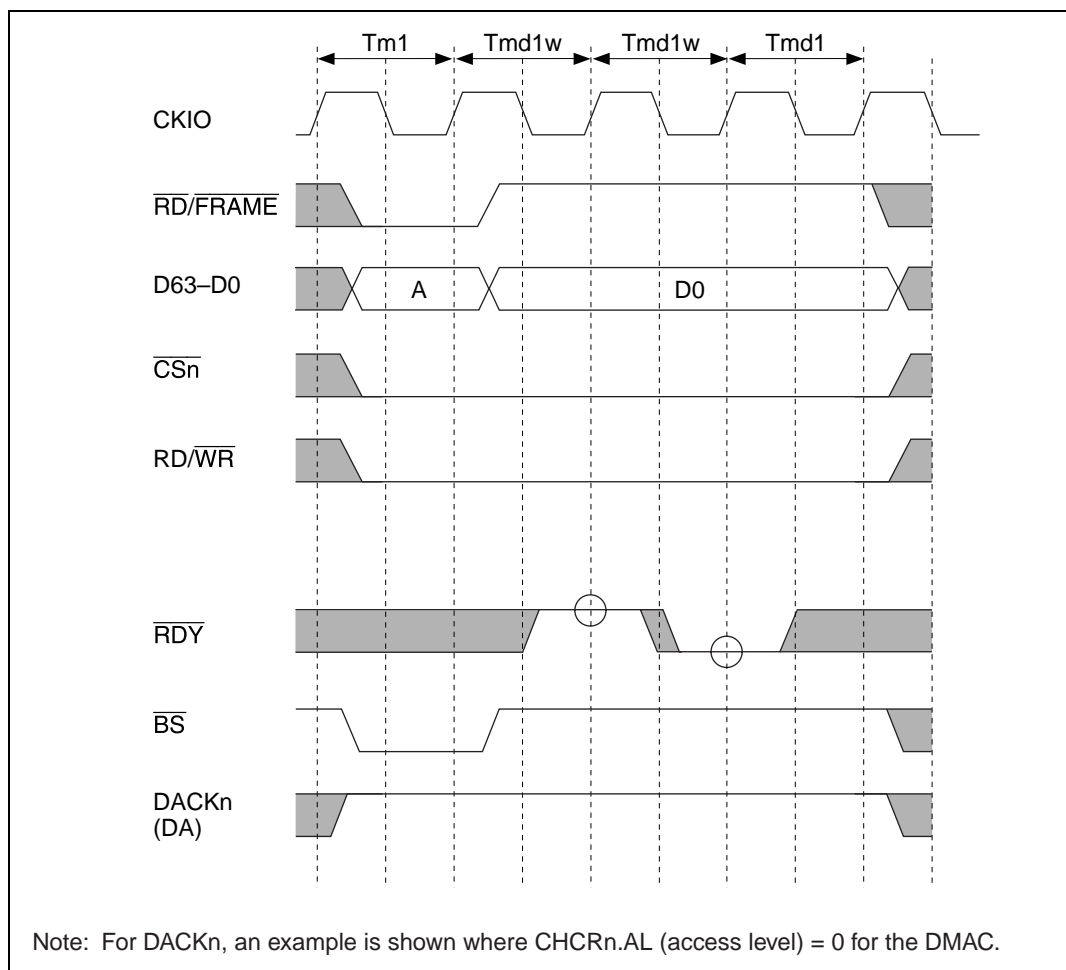
Figure 13.60 MPX Interface Timing 4 (Single Write, AnW = 1, One External Wait Inserted, Bus Width: 64 Bits)
