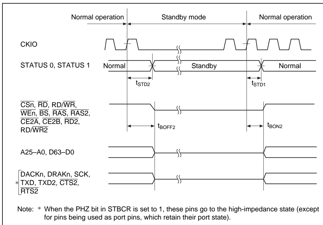
Figure 22.14 Pin Drive Timing for Standby Mode
