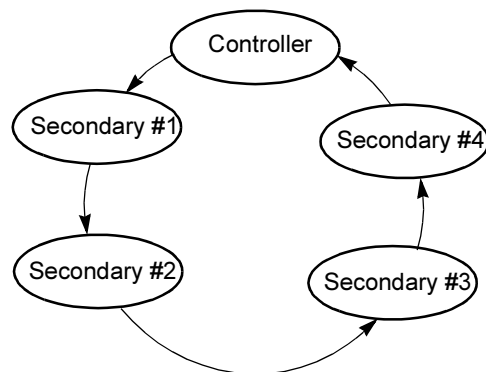
Figure 10. SDLC Loop
