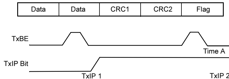
Figure 14. TxIP Latching
