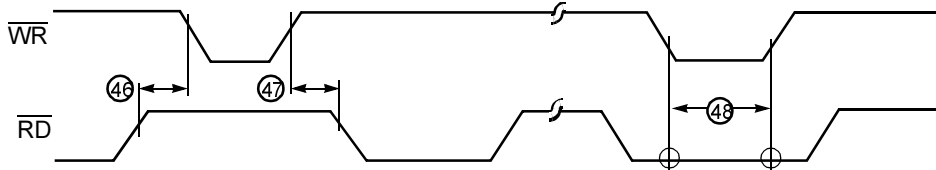
Figure 31. Z85230 Reset Timing Diagram
