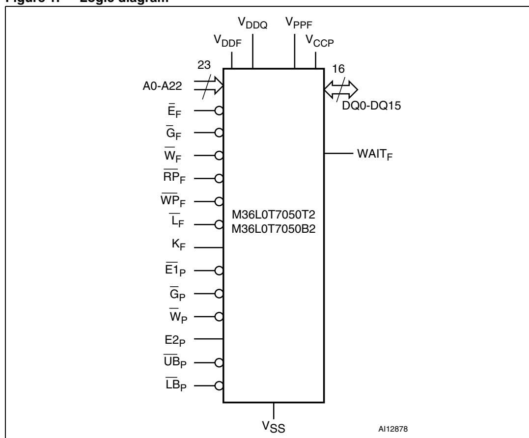
Figure 1. Logic diagram
