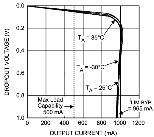
Dropout Voltage vs Output Current (Bypass mode, V_{IN} = \text{BYP} = 3.6V )
