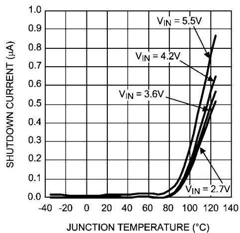
Shutdown Current vs Temperature (all EN = BYP , V_{CON} = SW = FB = 0V )
