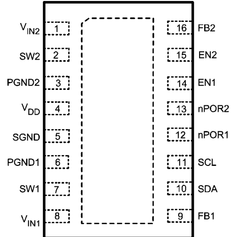
FIGURE 4. Top View
