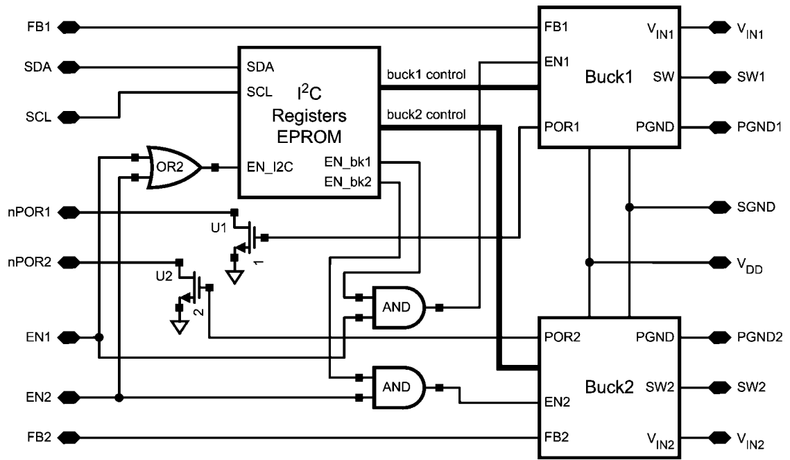
FIGURE 2. Functional Diagram
