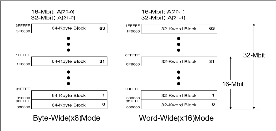
Figure 5. Memory Map
