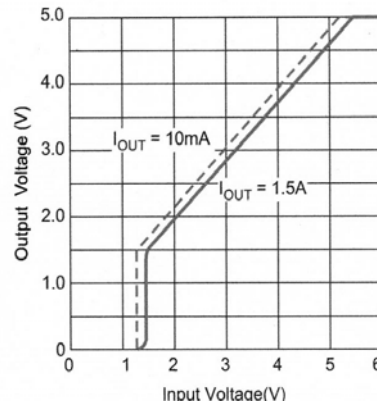
Figure 3. LM29150- 5.0 Dropout Characteristics
