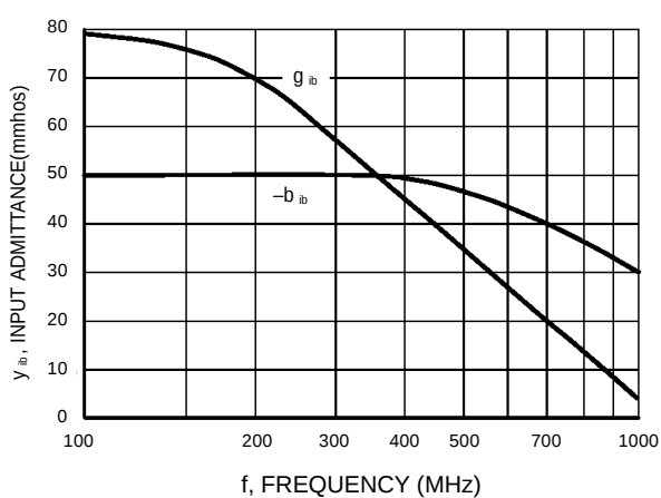
Figure 1. Rectangular Form
