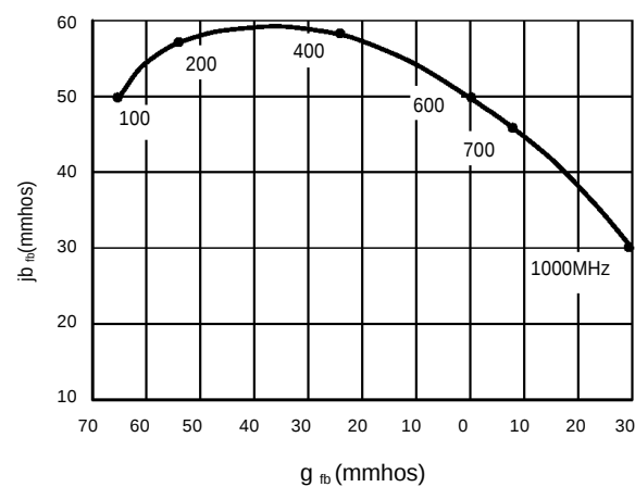
Figure 4. Polar Form
