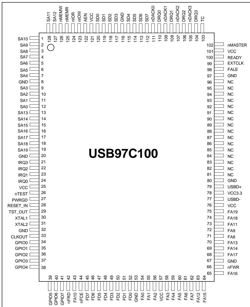
FIGURE 1 - PIN CONFIGURATION
