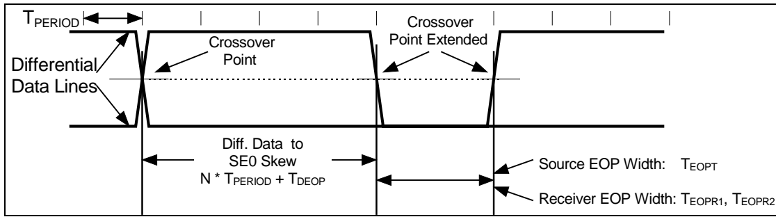
FIGURE 8 - DIFFERENTIAL TO EOP TRANSITION SKEW AND EOP WIDTH
