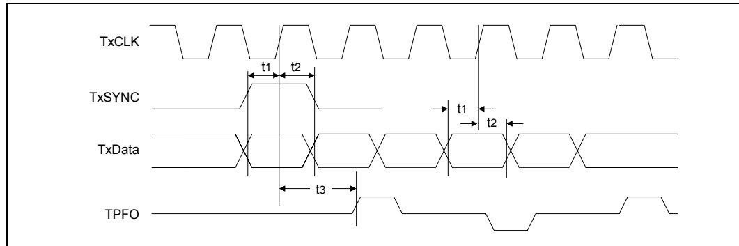
Figure 50. Intel® LXT9785/LXT9785E SS-SMII - 10BASE-T Transmit Timing
