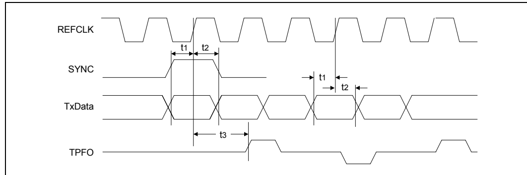
Figure 42. Intel® LXT9785/LXT9785E SMII - 100BASE-FX Transmit Timing
