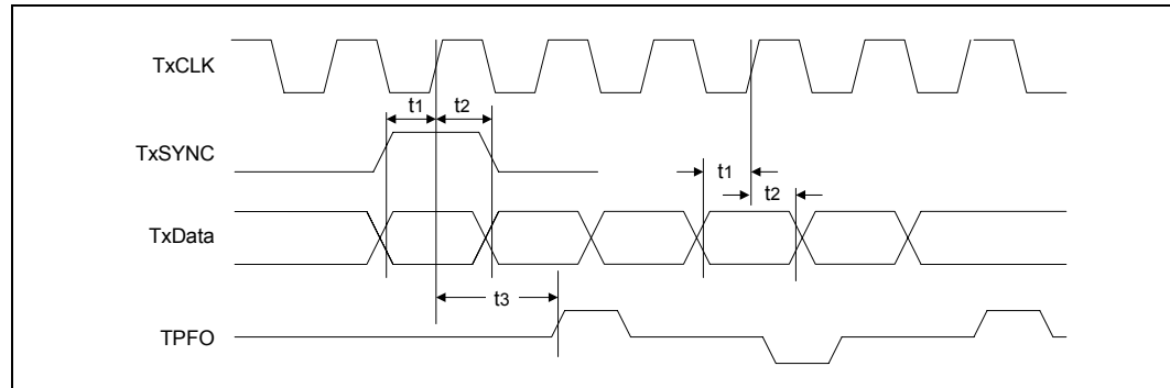
Figure 46. Intel® LXT9785/LXT9785E SS-SMII - 100BASE-TX Transmit Timing
