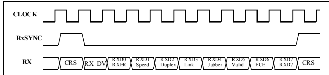
Figure 19. Intel® LXT9785/LXT9785E Serial MII Receive Synchronization
