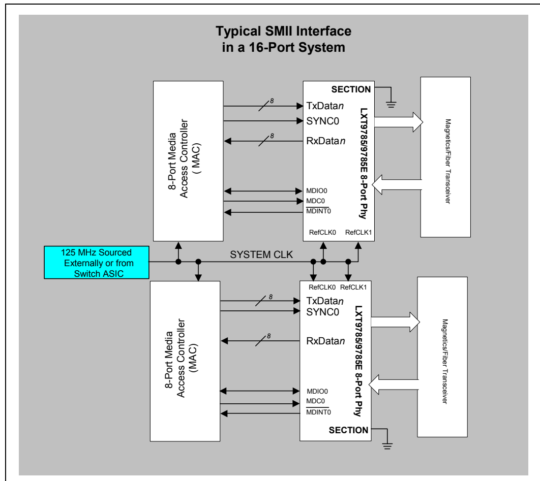
Figure 15. Intel® LXT9785/LXT9785E Typical SMII Interface Diagram
