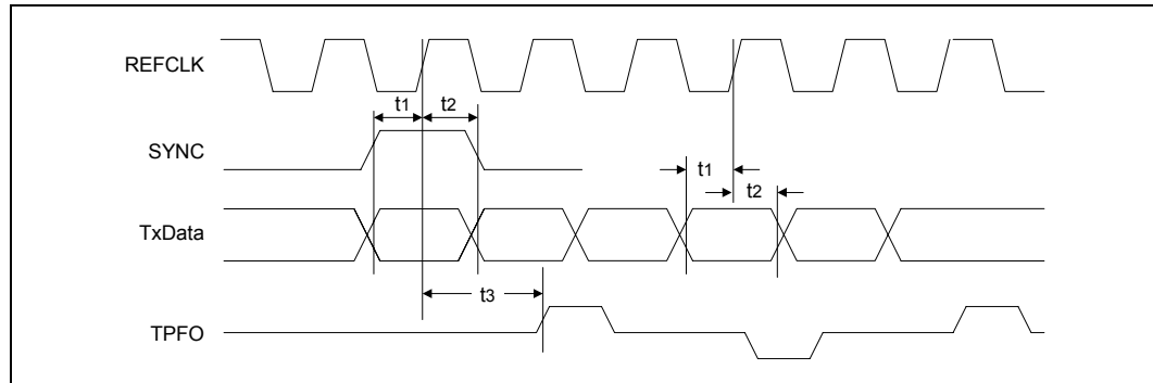
Figure 40. Intel® LXT9785/LXT9785E SMII - 100BASE-TX Transmit Timing
