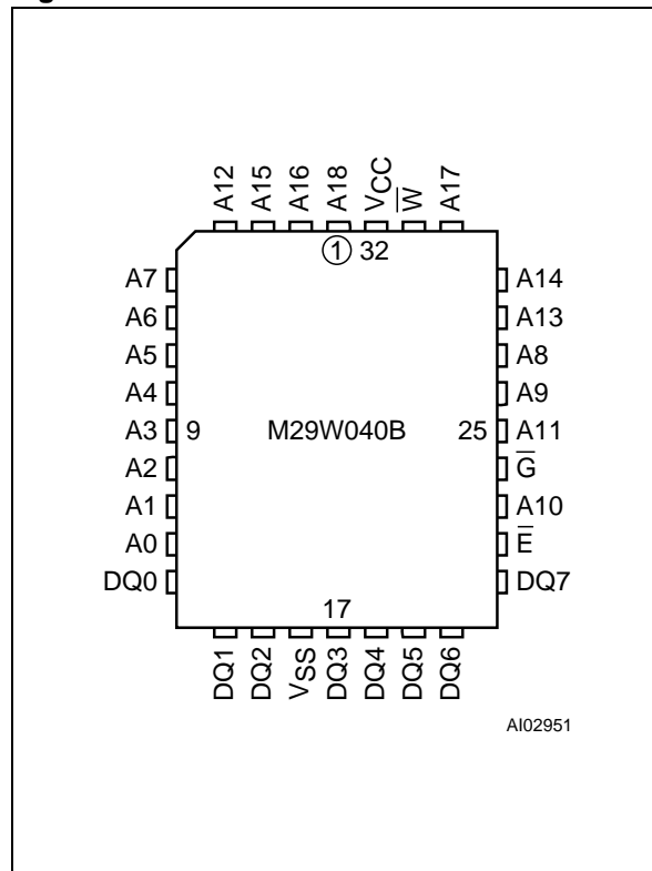
Figure 2. PLCC Connections
