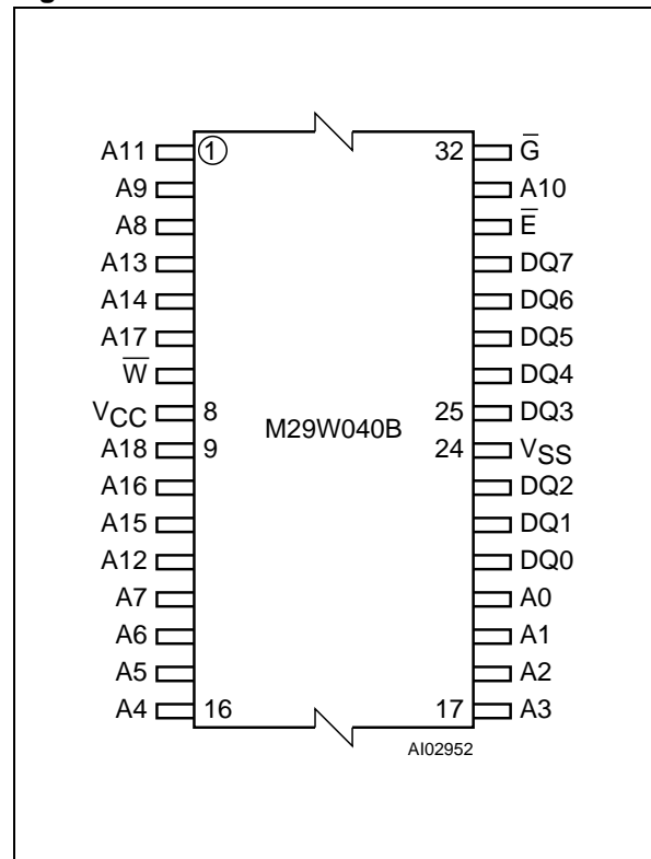
Figure 3. TSOP Connections
