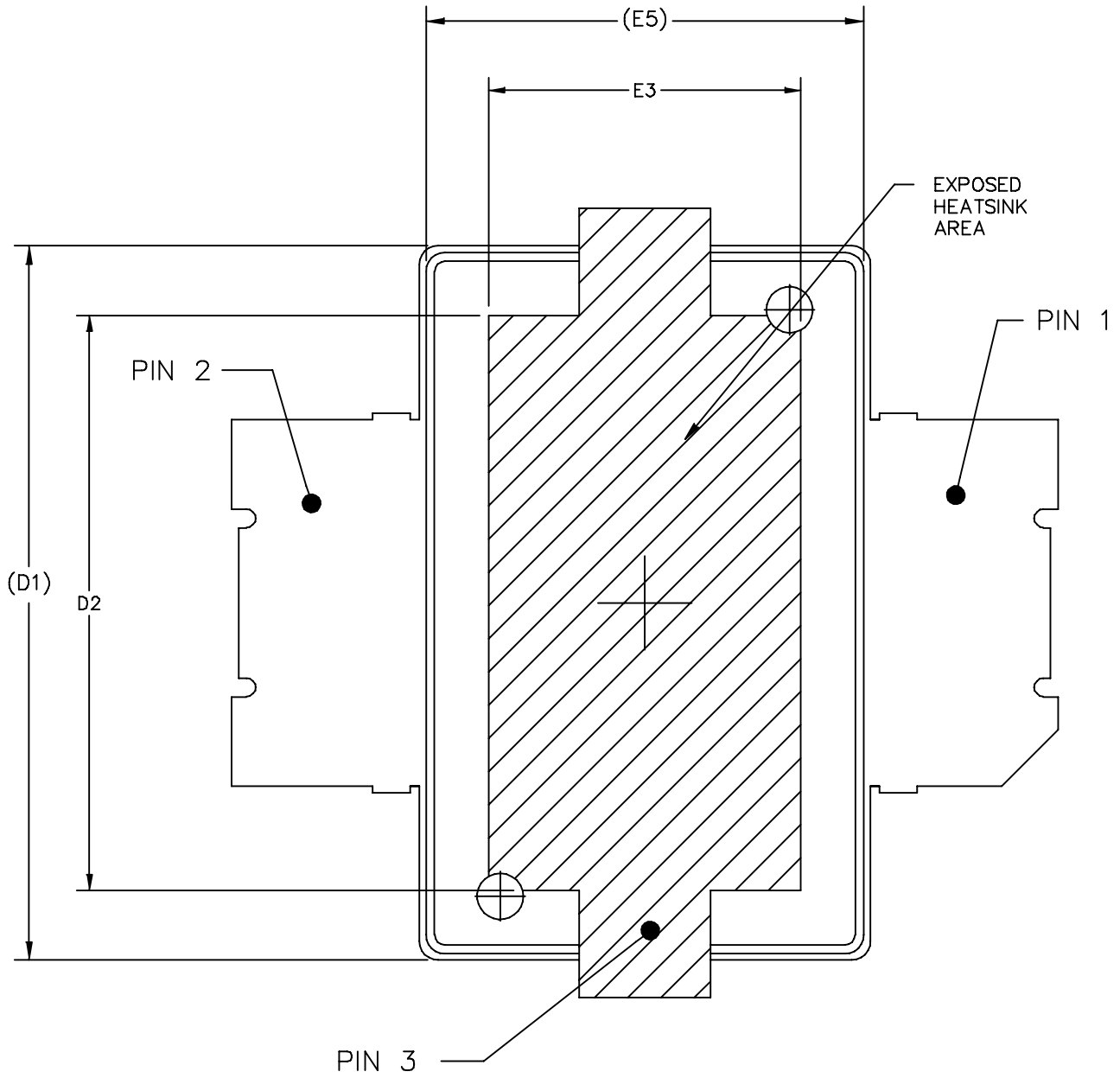
BOTTOM VIEW
