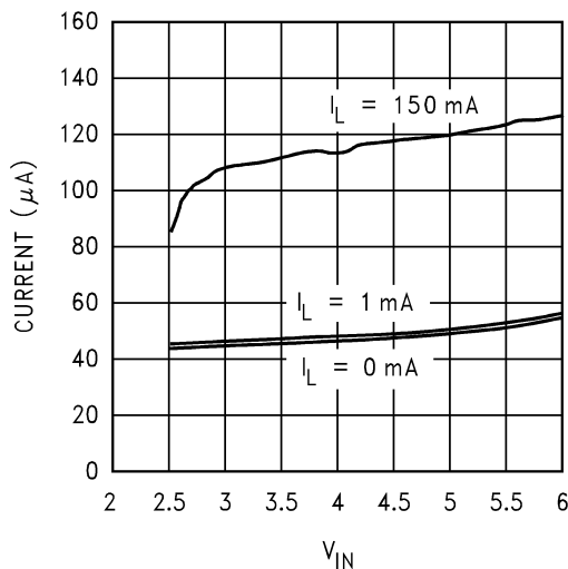
Ground Current vs V_{IN} @ -40^\circ\text{C}
