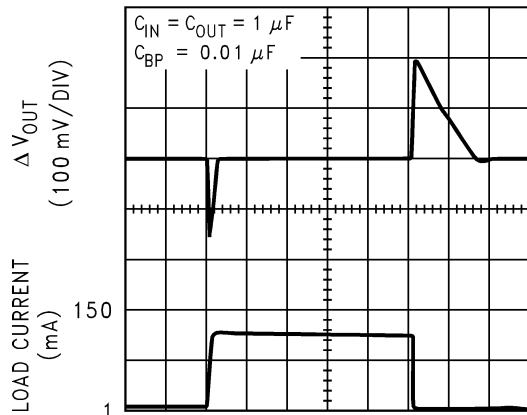
Load Transient Response ( V_{OUT} = 1.8\text{V} )
