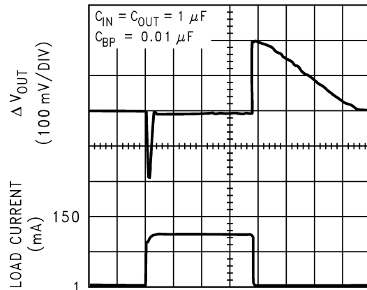
Load Transient Response ( V_{OUT} = 1.5\text{V} )
