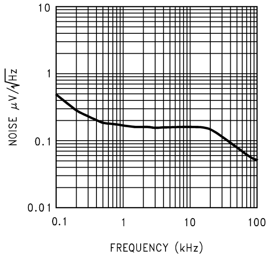
Output Noise Density V_{IN} = 4.2\text{V} V_{OUT} = 2.5\text{V}
