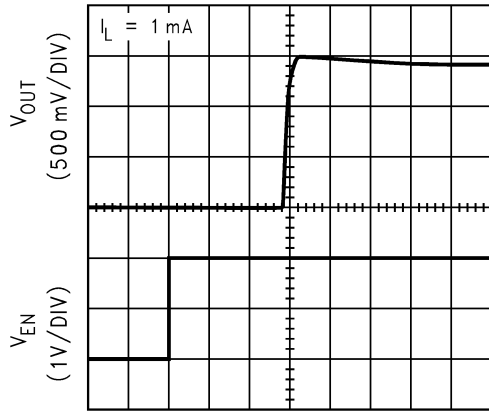
Enable Start-Up Time ( V_{OUT} = 1.5\text{V} )
