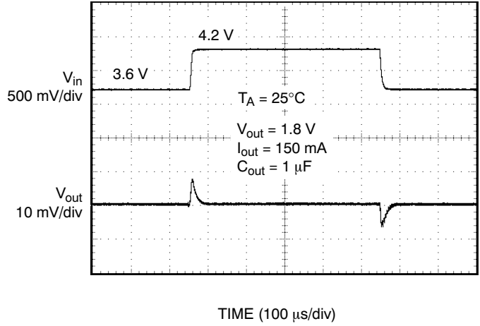
Figure 16. Line Transient
