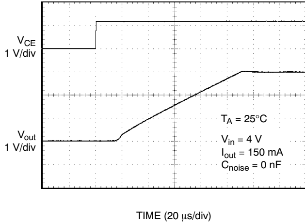
Figure 15. Enable Voltage and Output Voltage vs. Time (Start-Up)
