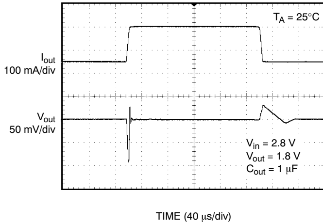
Figure 17. Load Transient
